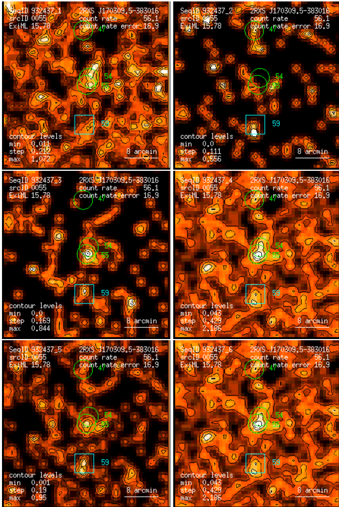
Figure 55: RASS 932437: detection 0055: band rate images, Gaussian filter: (1) PSPC channels 11 – 41, (2) 52 – 90, (3) 91 – 201, (4) 11 – 235, (5) 52 – 201, (6) 11 – 201. Broad band rates in counts/ks. Band rate contour levels in counts/ks/arcmin 2 .
