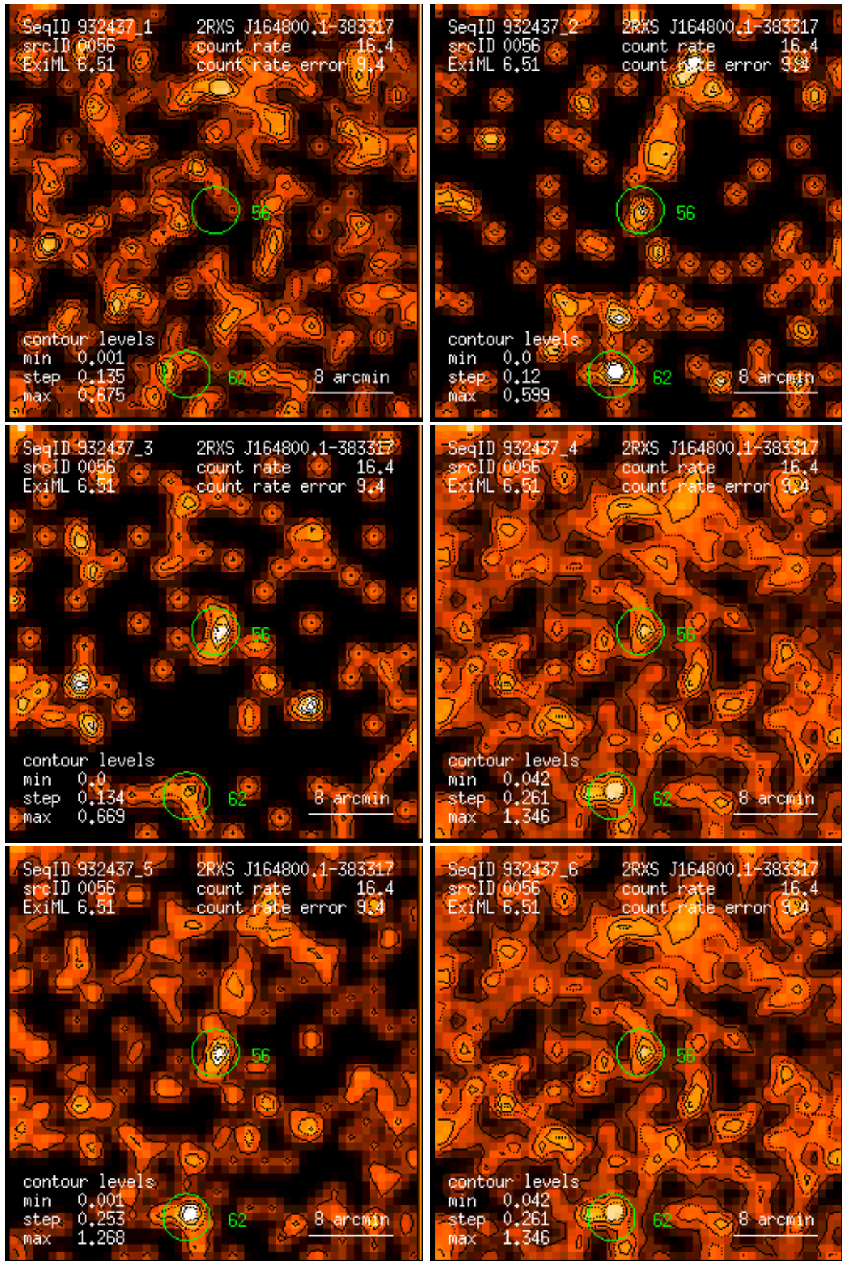
Figure 56: RASS 932437: detection 0056: band rate images, Gaussian filter: (1) PSPC channels 11 – 41, (2) 52 – 90, (3) 91 – 201, (4) 11 – 235, (5) 52 – 201, (6) 11 – 201. Broad band rates in counts/ks. Band rate contour levels in counts/ks/arcmin 2 .
