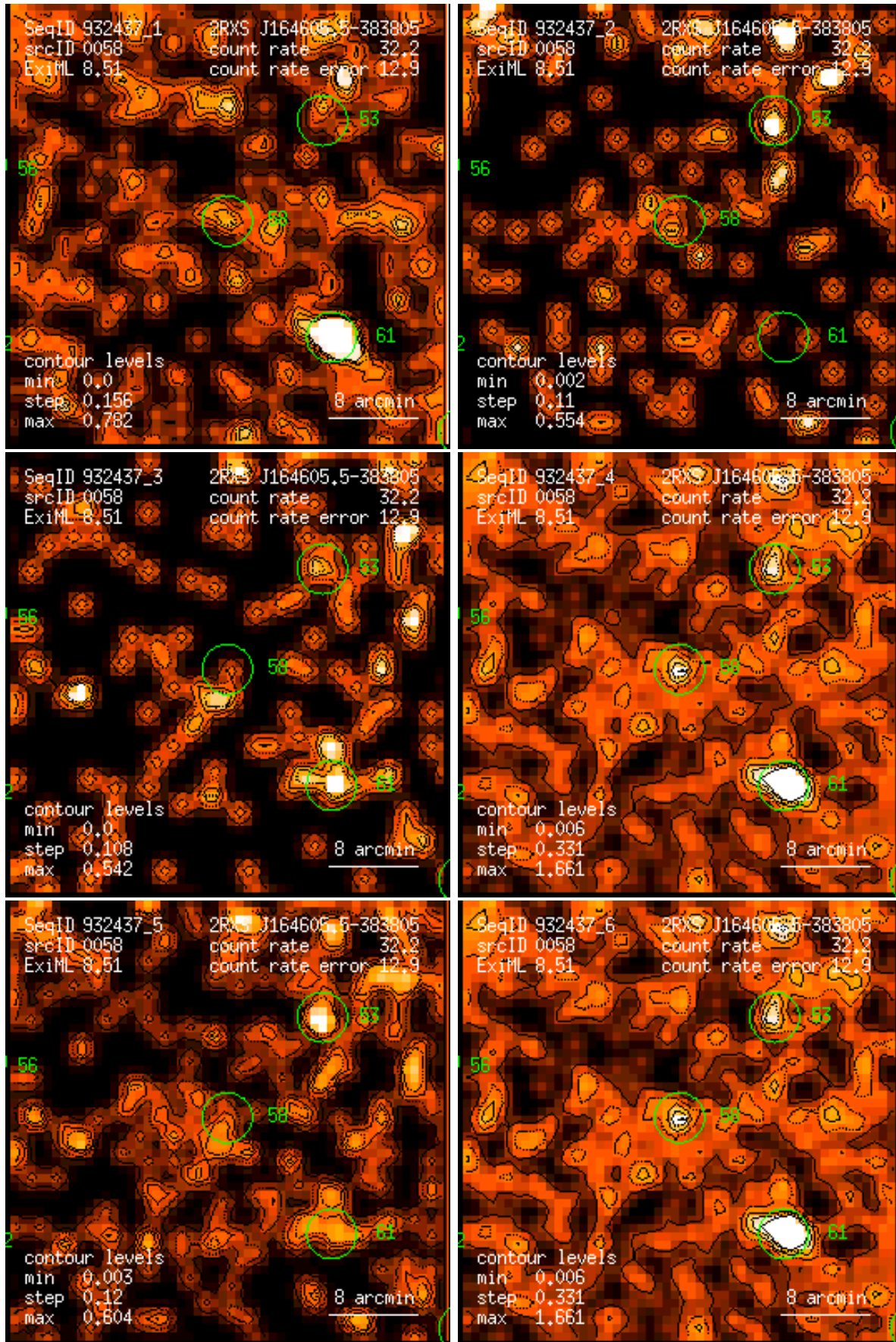
Figure 58: RASS 932437: detection 0058: band rate images, Gaussian filter: (1) PSPC channels 11 – 41, (2) 52 – 90, (3) 91 – 201, (4) 11 – 235, (5) 52 – 201, (6) 11 – 201. Broad band rates in counts/ks. Band rate contour levels in counts/ks/arcmin 2 .
