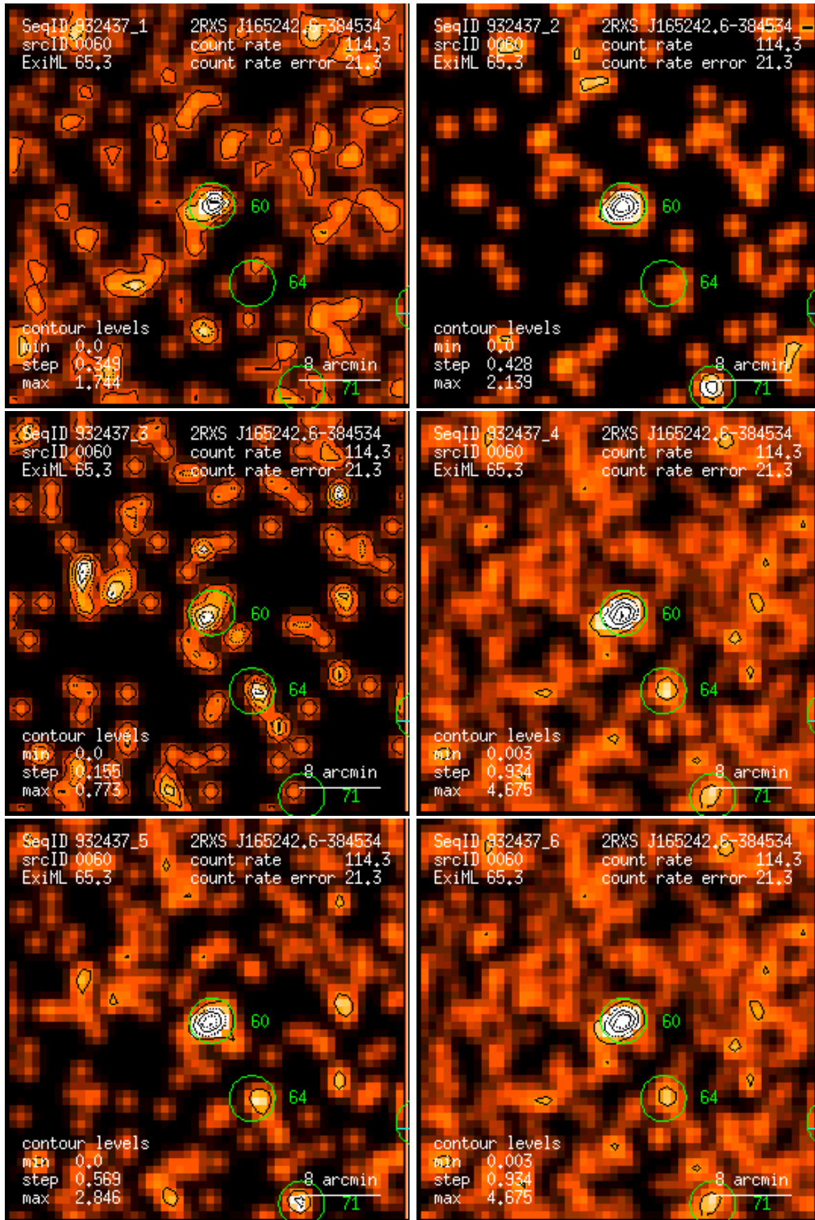
Figure 60: RASS 932437: detection 0060: band rate images, Gaussian filter: (1) PSPC channels 11 – 41, (2) 52 – 90, (3) 91 – 201, (4) 11 – 235, (5) 52 – 201, (6) 11 – 201. Broad band rates in counts/ks. Band rate contour levels in counts/ks/arcmin 2 .
