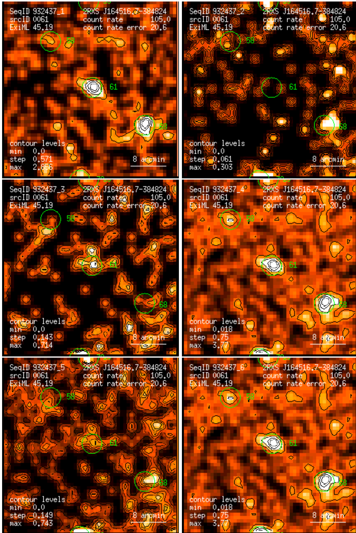
Figure 61: RASS 932437: detection 0061: band rate images, Gaussian filter: (1) PSPC channels 11 – 41, (2) 52 – 90, (3) 91 – 201, (4) 11 – 235, (5) 52 – 201, (6) 11 – 201. Broad band rates in counts/ks. Band rate contour levels in counts/ks/arcmin 2 .
