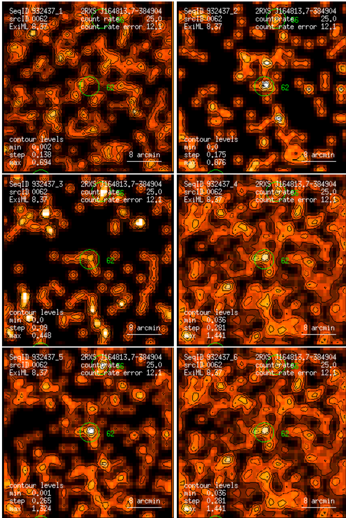
Figure 62: RASS 932437: detection 0062: band rate images, Gaussian filter: (1) PSPC channels 11 – 41, (2) 52 – 90, (3) 91 – 201, (4) 11 – 235, (5) 52 – 201, (6) 11 – 201. Broad band rates in counts/ks. Band rate contour levels in counts/ks/arcmin 2 .
