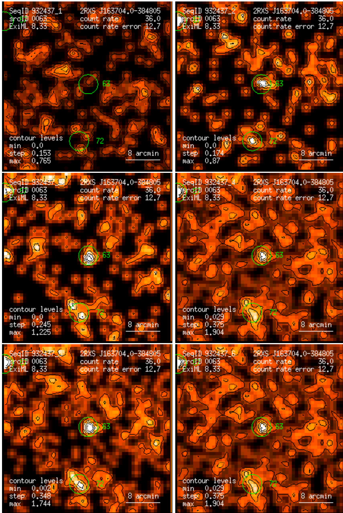
Figure 63: RASS 932437: detection 0063: band rate images, Gaussian filter: (1) PSPC channels 11 – 41, (2) 52 – 90, (3) 91 – 201, (4) 11 – 235, (5) 52 – 201, (6) 11 – 201. Broad band rates in counts/ks. Band rate contour levels in counts/ks/arcmin 2 .
