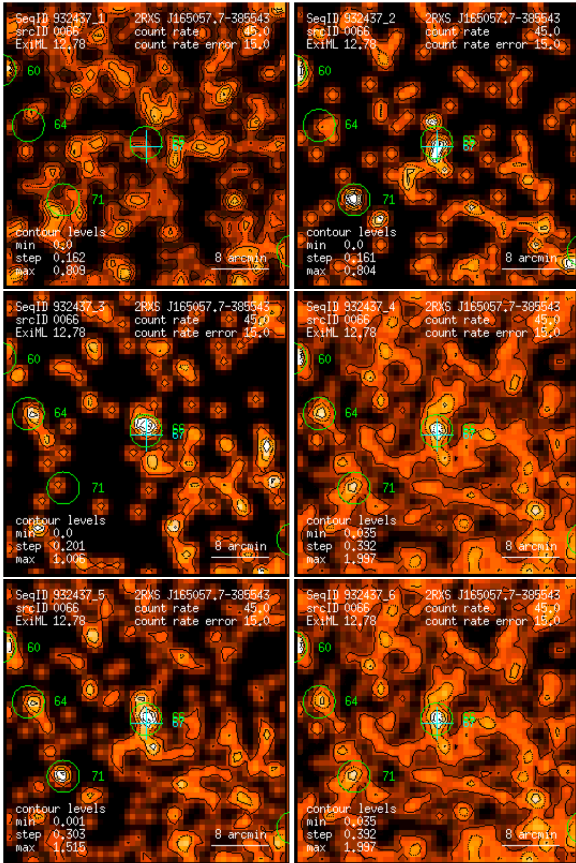
Figure 66: RASS 932437: detection 0066: band rate images, Gaussian filter: (1) PSPC channels 11 – 41, (2) 52 – 90, (3) 91 – 201, (4) 11 – 235, (5) 52 – 201, (6) 11 – 201. Broad band rates in counts/ks. Band rate contour levels in counts/ks/arcmin 2 .
