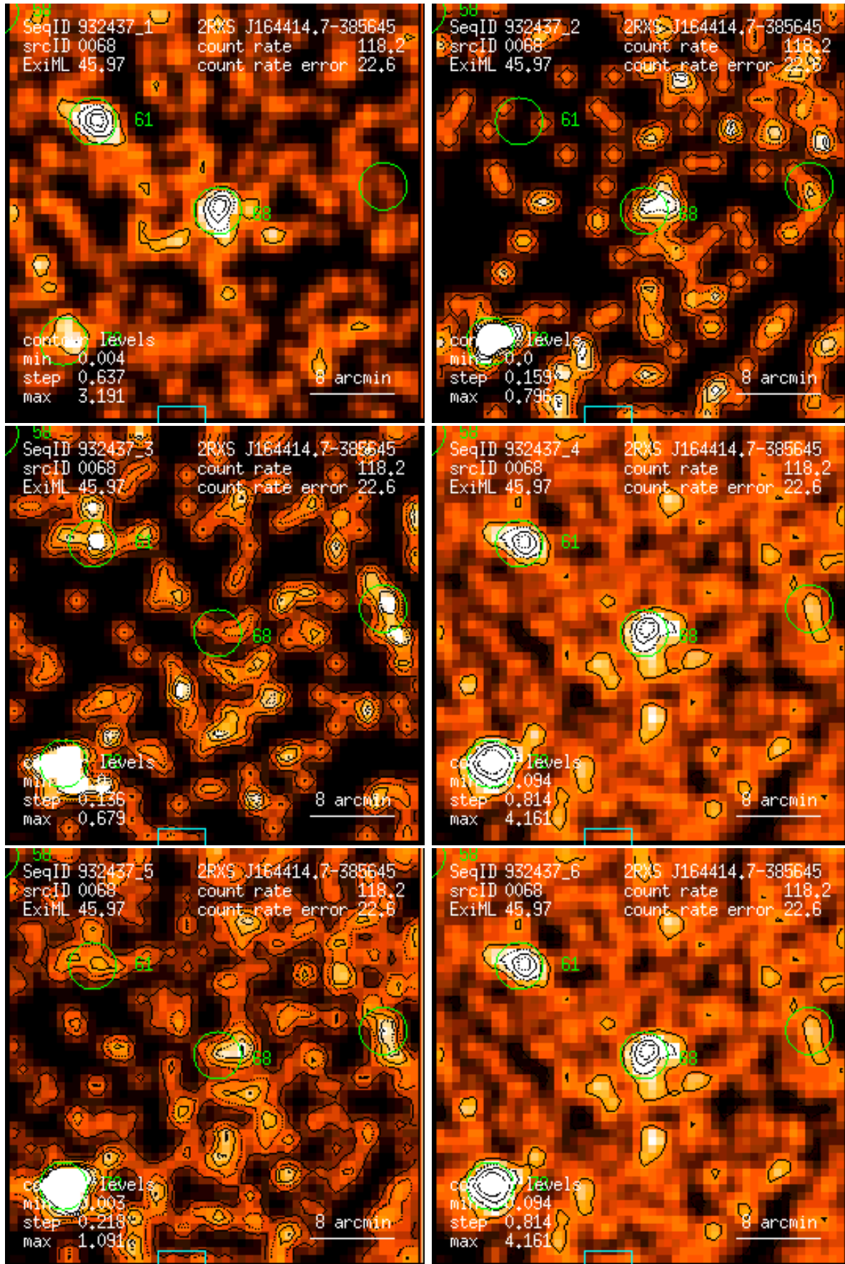
Figure 68: RASS 932437: detection 0068: band rate images, Gaussian filter: (1) PSPC channels 11 – 41, (2) 52 – 90, (3) 91 – 201, (4) 11 – 235, (5) 52 – 201, (6) 11 – 201. Broad band rates in counts/ks. Band rate contour levels in counts/ks/arcmin 2 .
