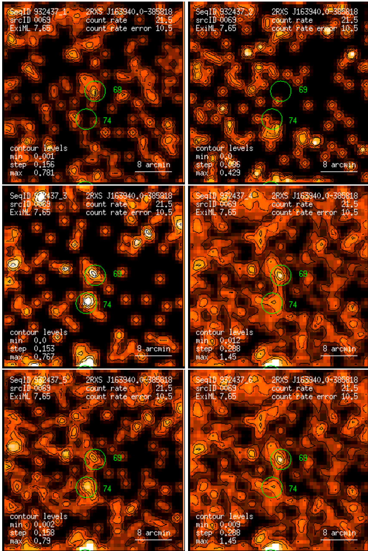
Figure 69: RASS 932437: detection 0069: band rate images, Gaussian filter: (1) PSPC channels 11 – 41, (2) 52 – 90, (3) 91 – 201, (4) 11 – 235, (5) 52 – 201, (6) 11 – 201. Broad band rates in counts/ks. Band rate contour levels in counts/ks/arcmin 2 .
