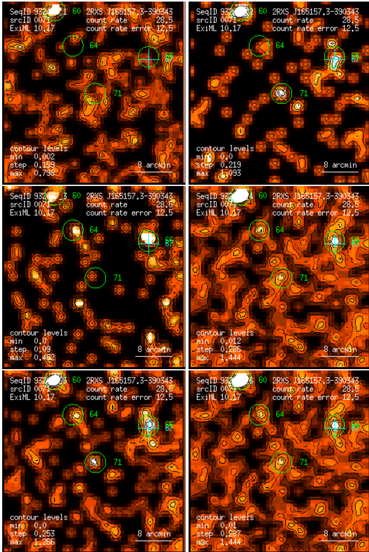
Figure 71: RASS 932437: detection 0071: band rate images, Gaussian filter: (1) PSPC channels 11 – 41, (2) 52 – 90, (3) 91 – 201, (4) 11 – 235, (5) 52 – 201, (6) 11 – 201. Broad band rates in counts/ks. Band rate contour levels in counts/ks/arcmin 2 .
