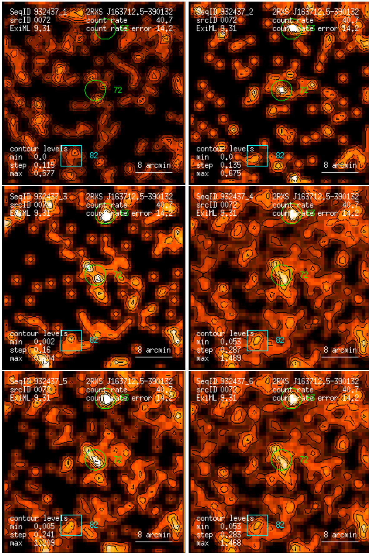
Figure 72: RASS 932437: detection 0072: band rate images, Gaussian filter: (1) PSPC channels 11 – 41, (2) 52 – 90, (3) 91 – 201, (4) 11 – 235, (5) 52 – 201, (6) 11 – 201. Broad band rates in counts/ks. Band rate contour levels in counts/ks/arcmin 2 .
