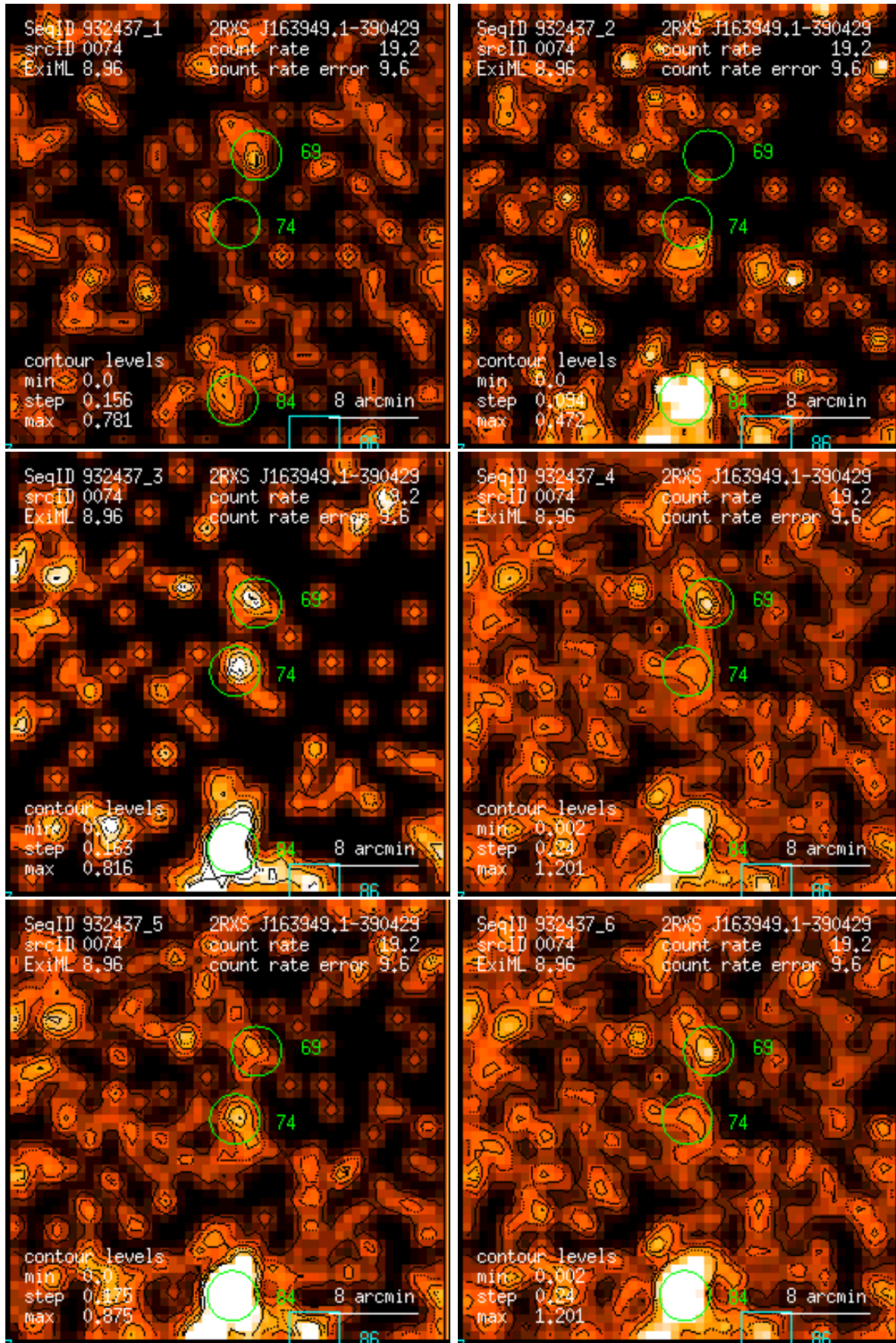
Figure 74: RASS 932437: detection 0074: band rate images, Gaussian filter: (1) PSPC channels 11 – 41, (2) 52 – 90, (3) 91 – 201, (4) 11 – 235, (5) 52 – 201, (6) 11 – 201. Broad band rates in counts/ks. Band rate contour levels in counts/ks/arcmin 2 .
