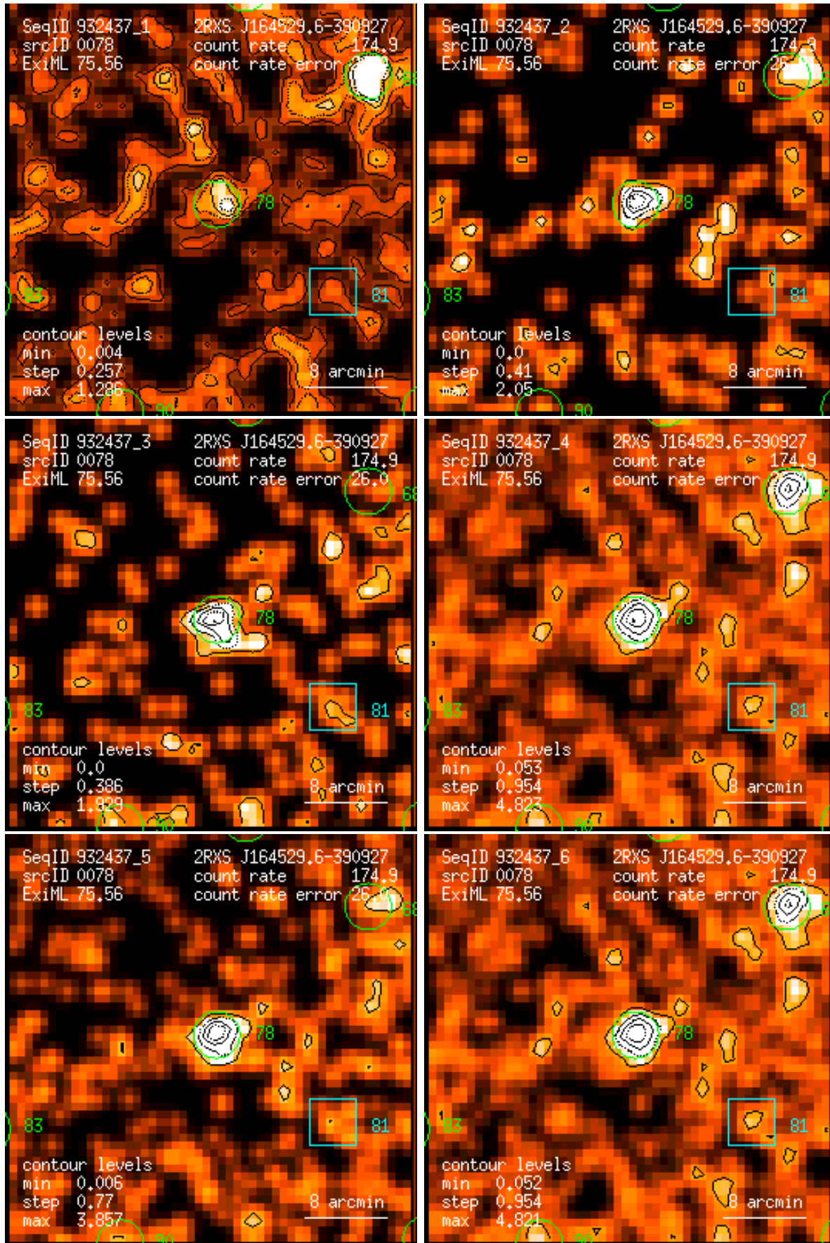
Figure 78: RASS 932437: detection 0078: band rate images, Gaussian filter: (1) PSPC channels 11 – 41, (2) 52 – 90, (3) 91 – 201, (4) 11 – 235, (5) 52 – 201, (6) 11 – 201. Broad band rates in counts/ks. Band rate contour levels in counts/ks/arcmin 2 .
