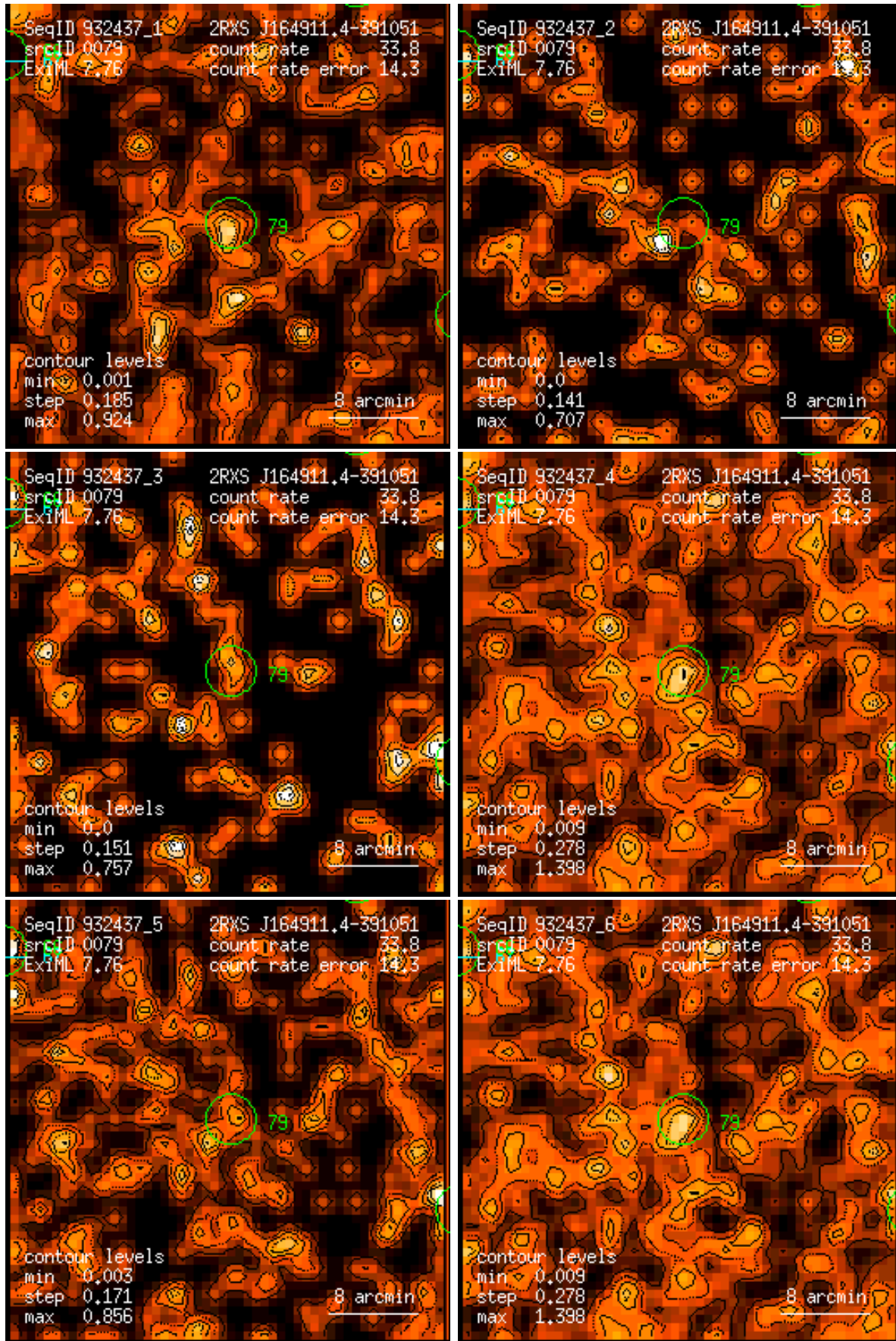
Figure 79: RASS 932437: detection 0079: band rate images, Gaussian filter: (1) PSPC channels 11 – 41, (2) 52 – 90, (3) 91 – 201, (4) 11 – 235, (5) 52 – 201, (6) 11 – 201. Broad band rates in counts/ks. Band rate contour levels in counts/ks/arcmin 2 .
