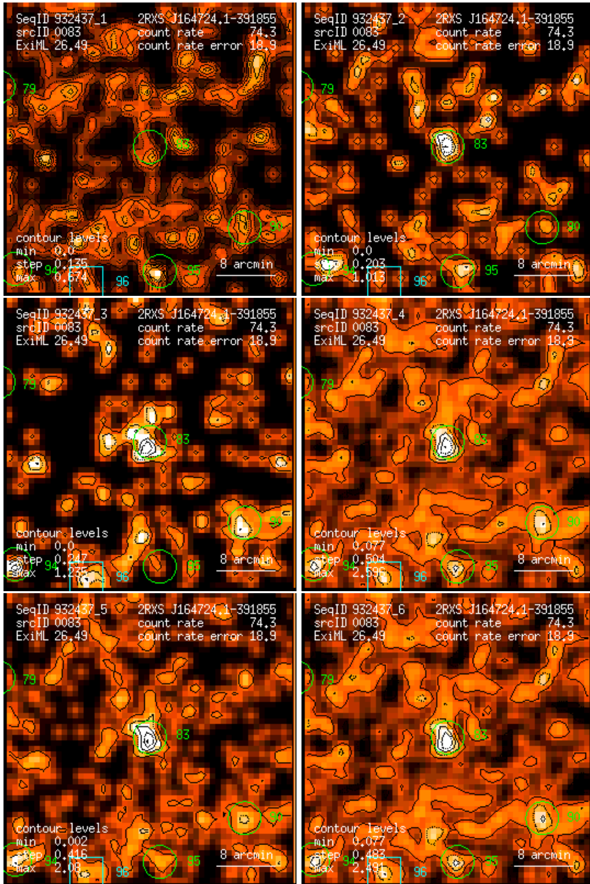
Figure 83: RASS 932437: detection 0083: band rate images, Gaussian filter: (1) PSPC channels 11 – 41, (2) 52 – 90, (3) 91 – 201, (4) 11 – 235, (5) 52 – 201, (6) 11 – 201. Broad band rates in counts/ks. Band rate contour levels in counts/ks/arcmin 2 .
