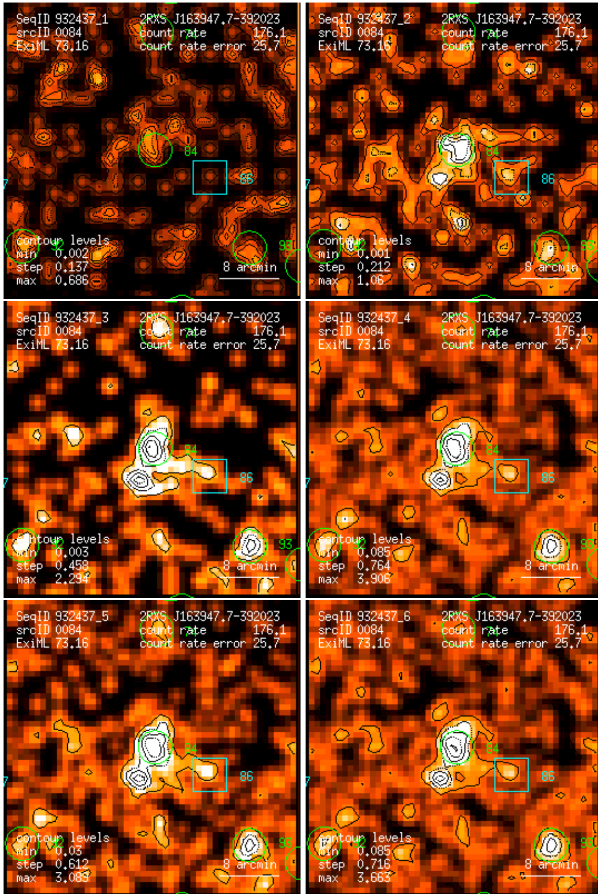
Figure 84: RASS 932437: detection 0084: band rate images, Gaussian filter: (1) PSPC channels 11 – 41, (2) 52 – 90, (3) 91 – 201, (4) 11 – 235, (5) 52 – 201, (6) 11 – 201. Broad band rates in counts/ks. Band rate contour levels in counts/ks/arcmin 2 .
