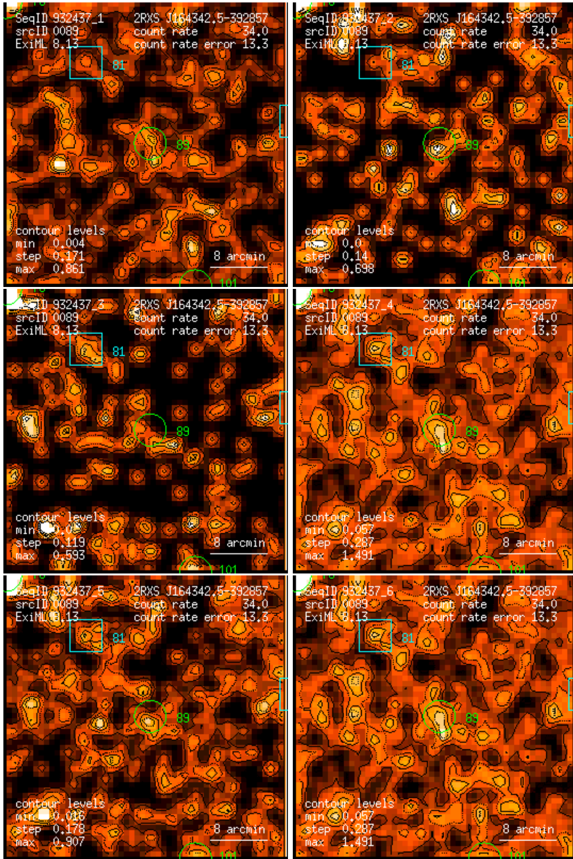
Figure 89: RASS 932437: detection 0089: band rate images, Gaussian filter: (1) PSPC channels 11 – 41, (2) 52 – 90, (3) 91 – 201, (4) 11 – 235, (5) 52 – 201, (6) 11 – 201. Broad band rates in counts/ks. Band rate contour levels in counts/ks/arcmin 2 .
