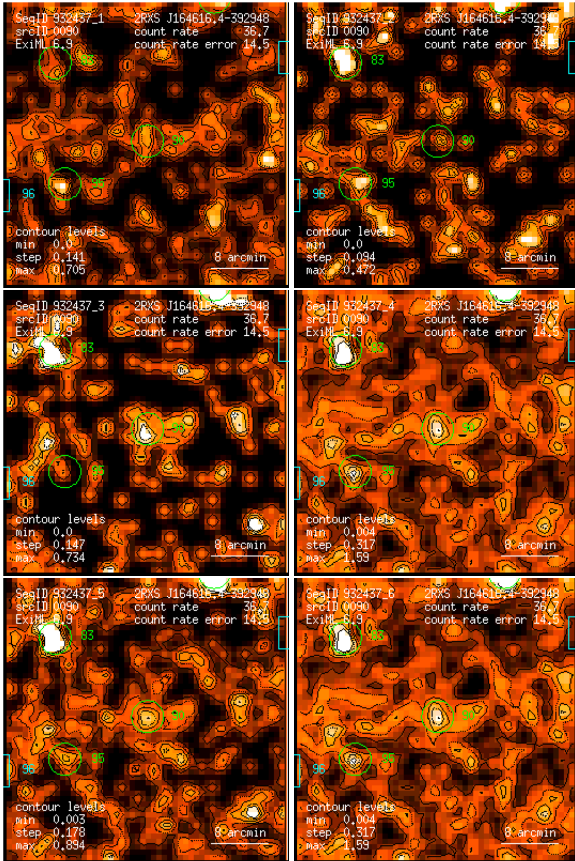
Figure 90: RASS 932437: detection 0090: band rate images, Gaussian filter: (1) PSPC channels 11 – 41, (2) 52 – 90, (3) 91 – 201, (4) 11 – 235, (5) 52 – 201, (6) 11 – 201. Broad band rates in counts/ks. Band rate contour levels in counts/ks/arcmin 2 .
