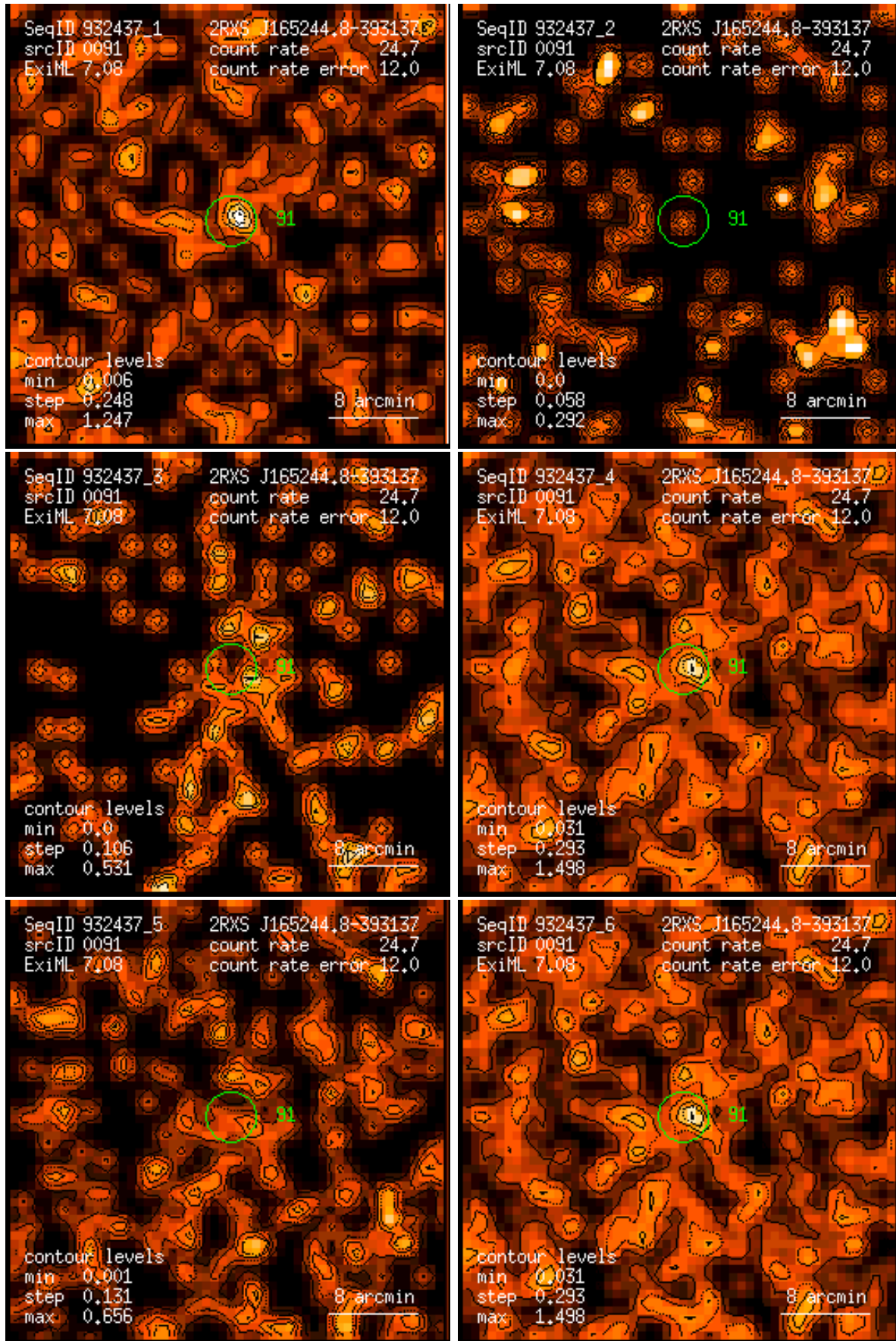
Figure 91: RASS 932437: detection 0091: band rate images, Gaussian filter: (1) PSPC channels 11 – 41, (2) 52 – 90, (3) 91 – 201, (4) 11 – 235, (5) 52 – 201, (6) 11 – 201. Broad band rates in counts/ks. Band rate contour levels in counts/ks/arcmin 2 .
