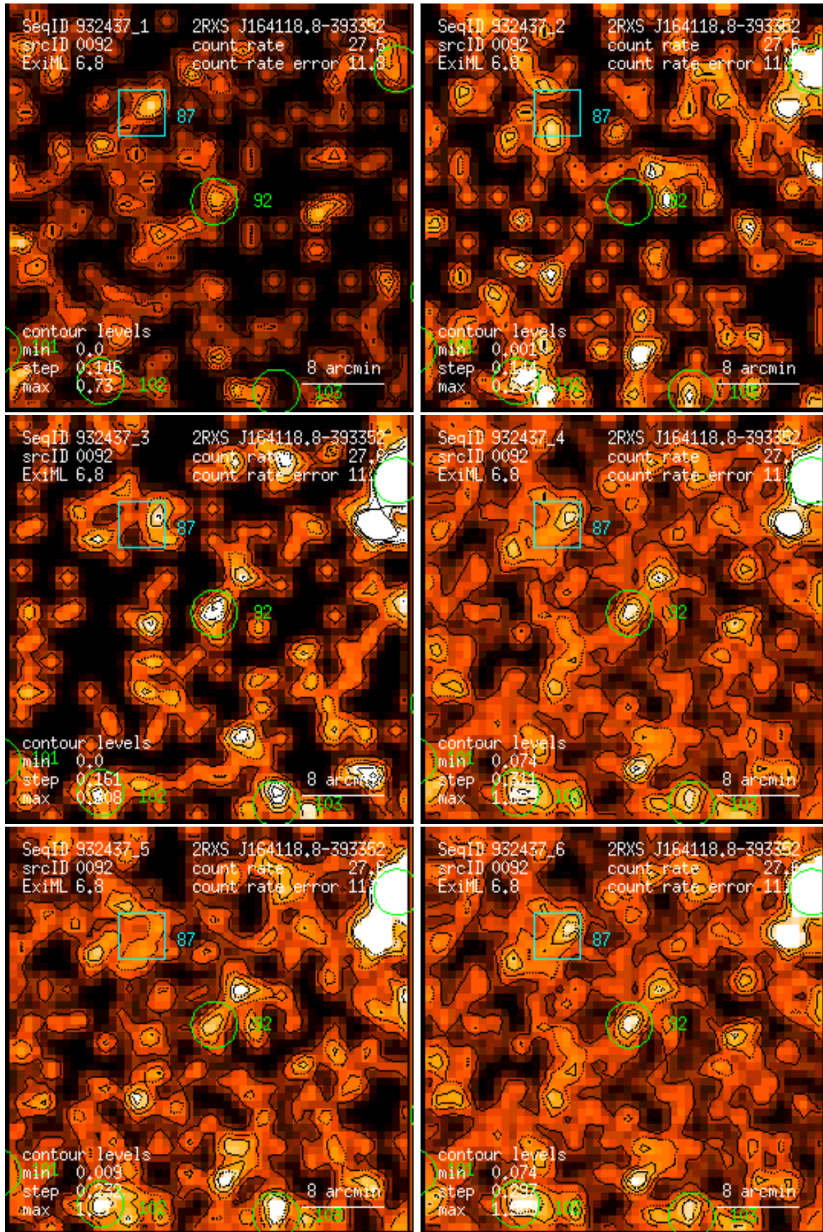
Figure 92: RASS 932437: detection 0092: band rate images, Gaussian filter: (1) PSPC channels 11 – 41, (2) 52 – 90, (3) 91 – 201, (4) 11 – 235, (5) 52 – 201, (6) 11 – 201. Broad band rates in counts/ks. Band rate contour levels in counts/ks/arcmin 2 .
