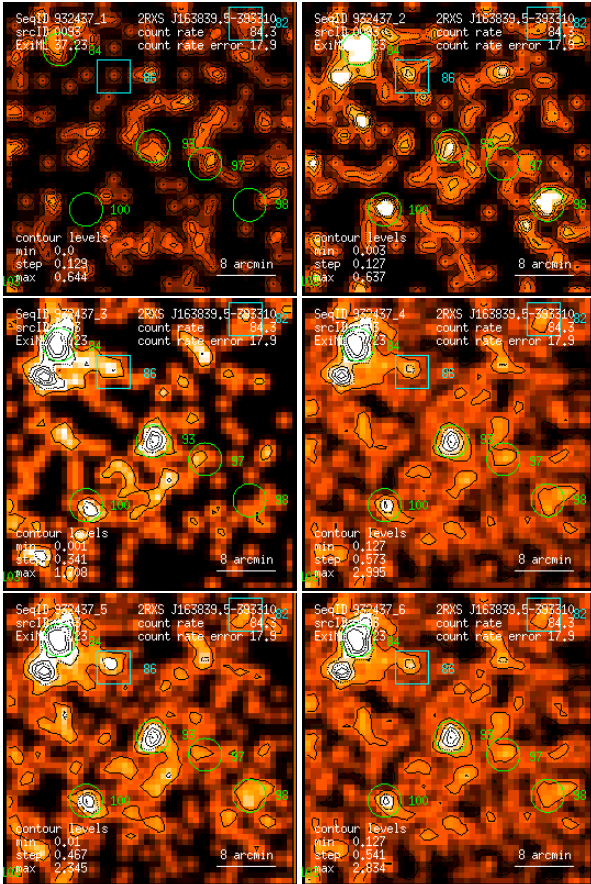
Figure 93: RASS 932437: detection 0093: band rate images, Gaussian filter: (1) PSPC channels 11 – 41, (2) 52 – 90, (3) 91 – 201, (4) 11 – 235, (5) 52 – 201, (6) 11 – 201. Broad band rates in counts/ks. Band rate contour levels in counts/ks/arcmin 2 .
