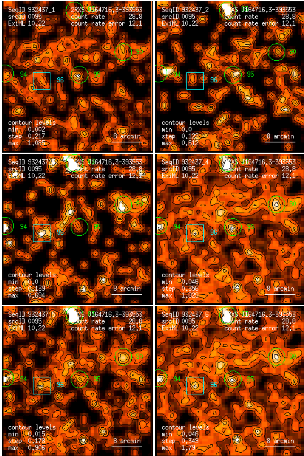
Figure 95: RASS 932437: detection 0095: band rate images, Gaussian filter: (1) PSPC channels 11 – 41, (2) 52 – 90, (3) 91 – 201, (4) 11 – 235, (5) 52 – 201, (6) 11 – 201. Broad band rates in counts/ks. Band rate contour levels in counts/ks/arcmin 2 .
