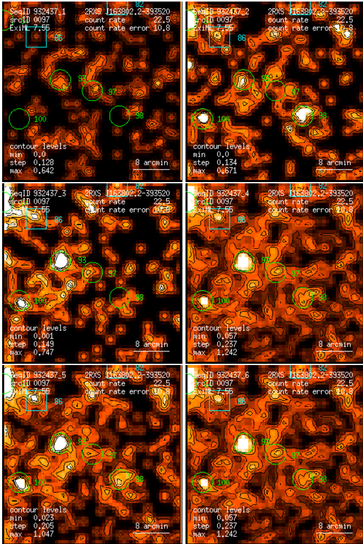
Figure 97: RASS 932437: detection 0097: band rate images, Gaussian filter: (1) PSPC channels 11 – 41, (2) 52 – 90, (3) 91 – 201, (4) 11 – 235, (5) 52 – 201, (6) 11 – 201. Broad band rates in counts/ks. Band rate contour levels in counts/ks/arcmin 2 .
