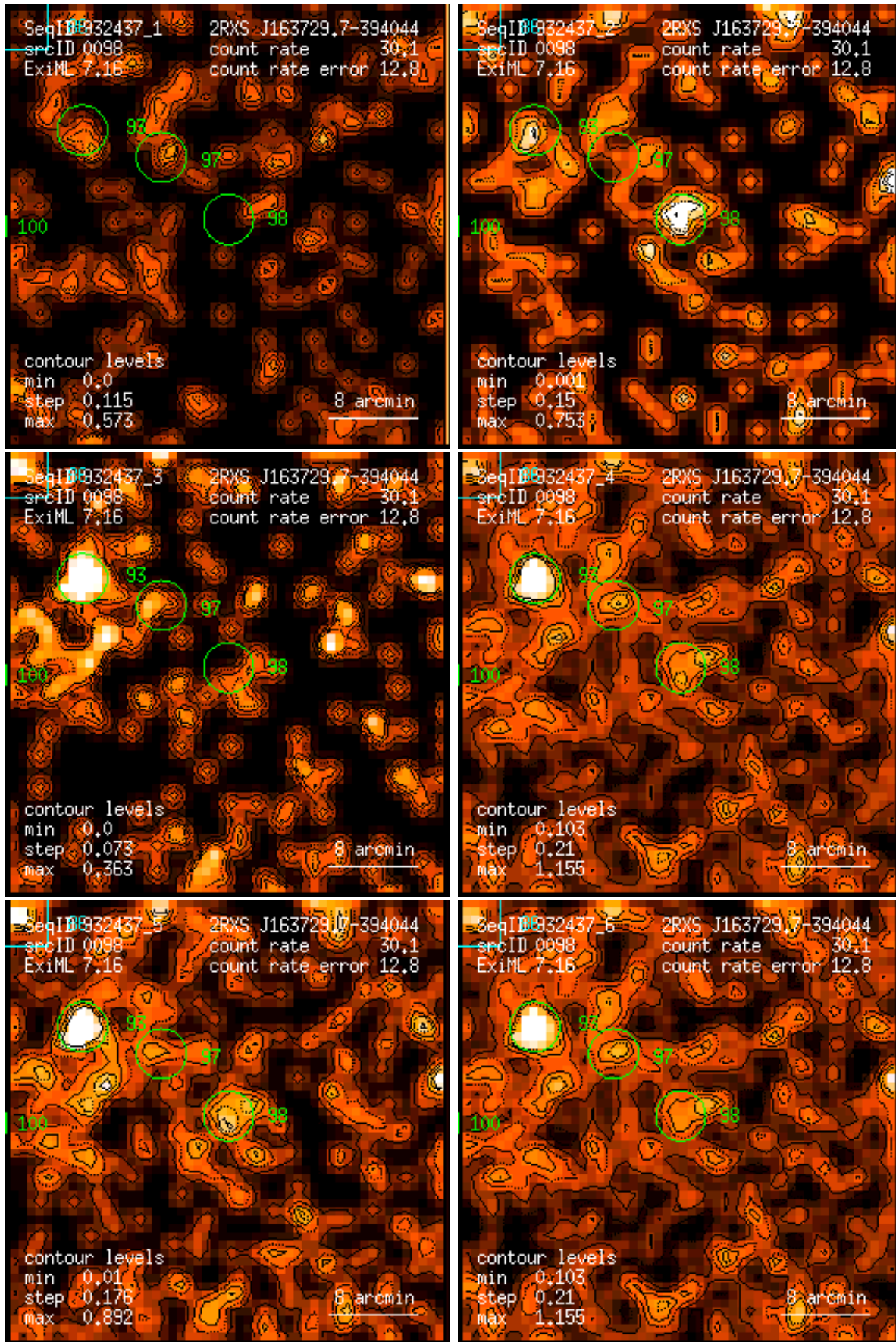
Figure 98: RASS 932437: detection 0098: band rate images, Gaussian filter: (1) PSPC channels 11 – 41, (2) 52 – 90, (3) 91 – 201, (4) 11 – 235, (5) 52 – 201, (6) 11 – 201. Broad band rates in counts/ks. Band rate contour levels in counts/ks/arcmin 2 .
