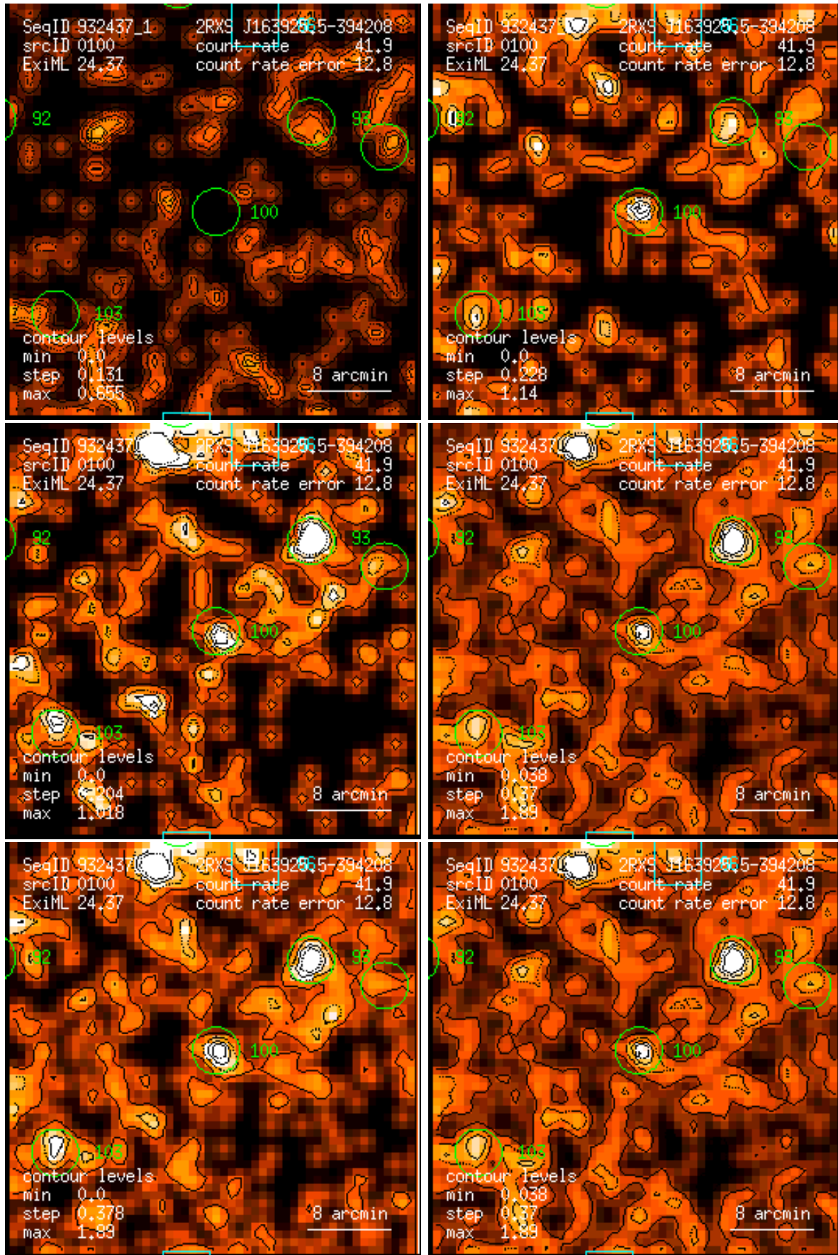
Figure 100: RASS 932437: detection 0100: band rate images, Gaussian filter: (1) PSPC channels 11 – 41, (2) 52 – 90, (3) 91 – 201, (4) 11 – 235, (5) 52 – 201, (6) 11 – 201. Broad band rates in counts/ks. Band rate contour levels in counts/ks/arcmin 2 .
