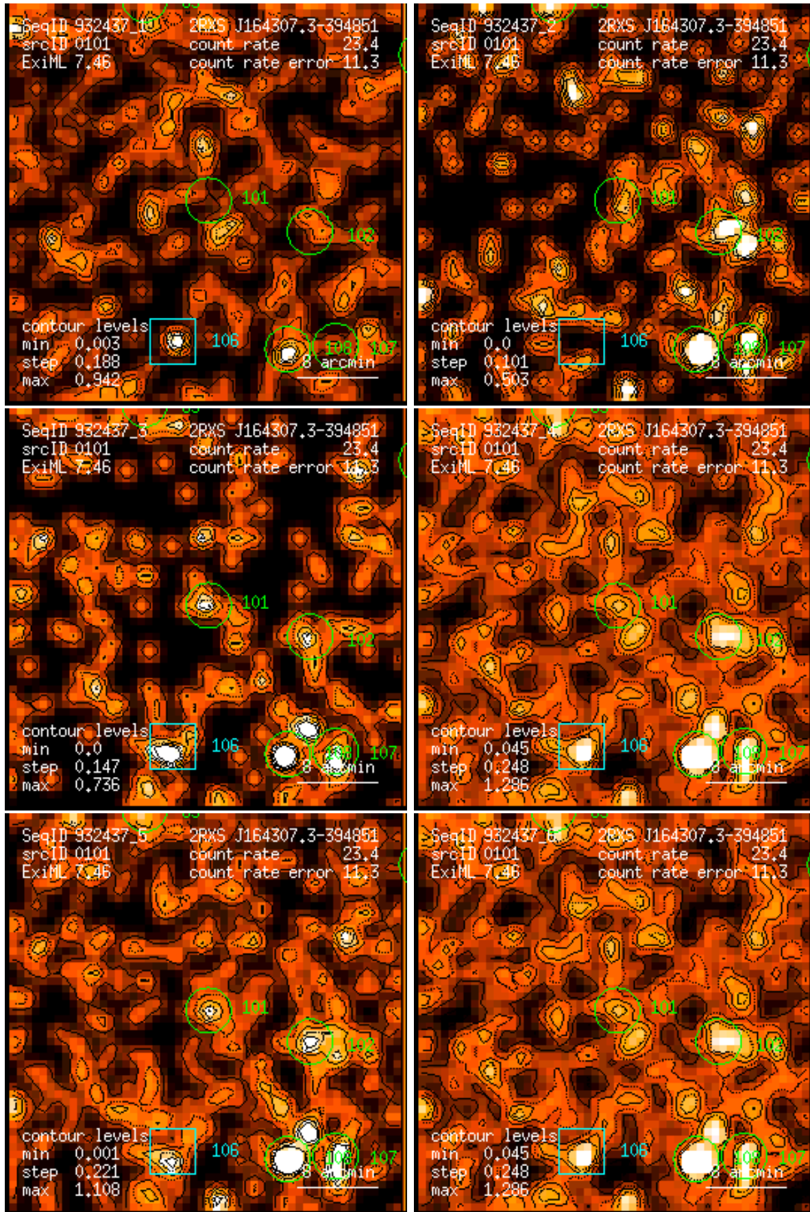
Figure 101: RASS 932437: detection 0101: band rate images, Gaussian filter: (1) PSPC channels 11 – 41, (2) 52 – 90, (3) 91 – 201, (4) 11 – 235, (5) 52 – 201, (6) 11 – 201. Broad band rates in counts/ks. Band rate contour levels in counts/ks/arcmin 2 .
