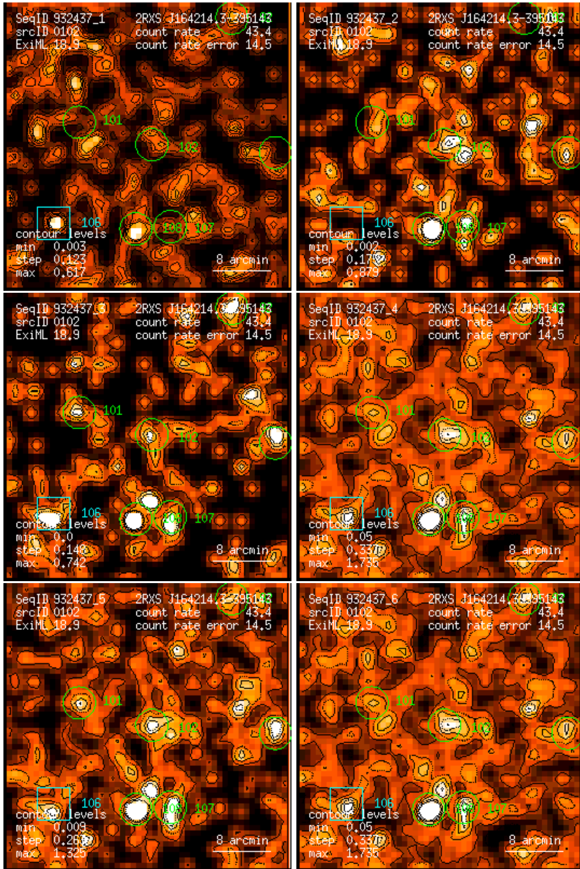
Figure 102: RASS 932437: detection 0102: band rate images, Gaussian filter: (1) PSPC channels 11 – 41, (2) 52 – 90, (3) 91 – 201, (4) 11 – 235, (5) 52 – 201, (6) 11 – 201. Broad band rates in counts/ks. Band rate contour levels in counts/ks/arcmin 2 .
