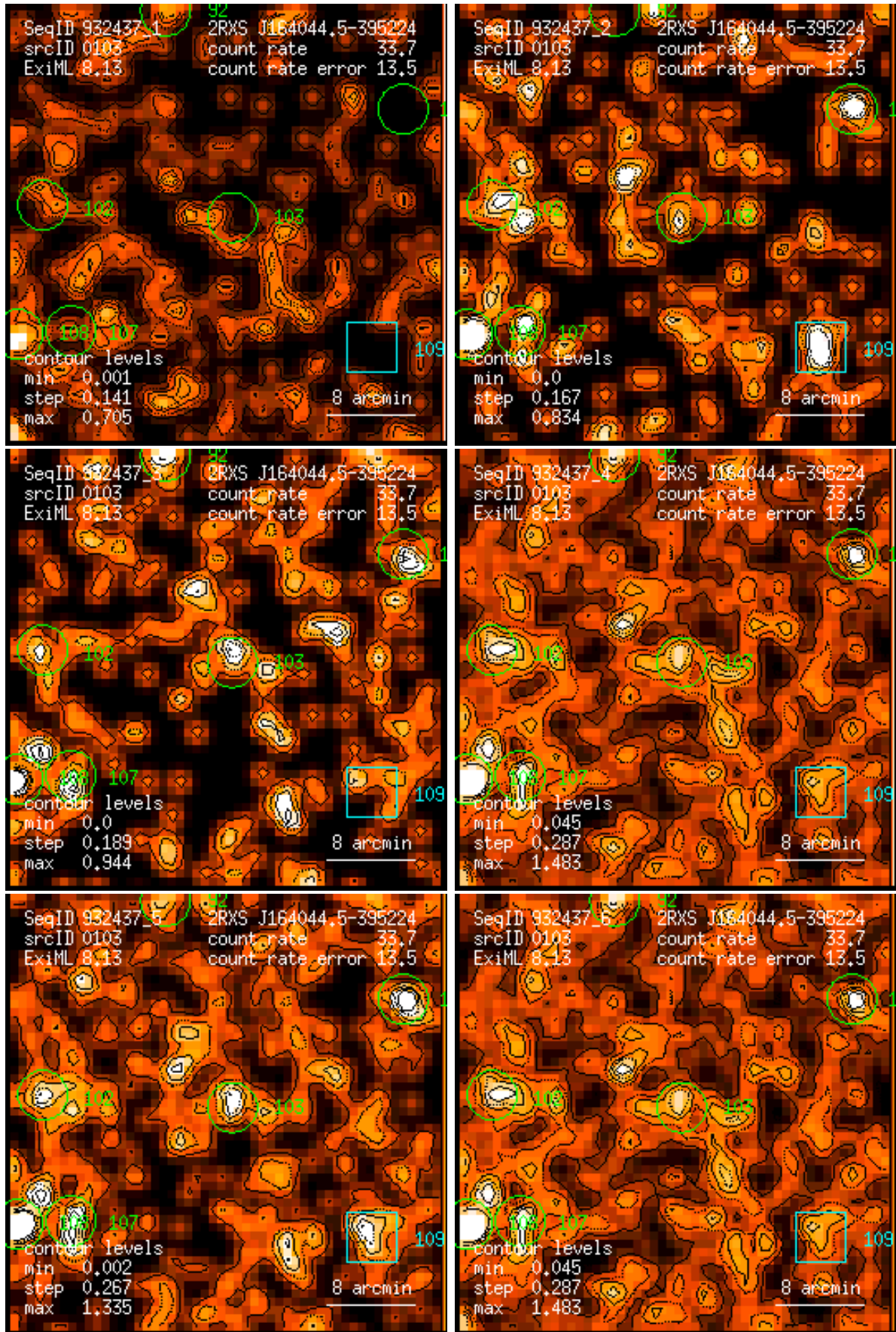
Figure 103: RASS 932437: detection 0103: band rate images, Gaussian filter: (1) PSPC channels 11 – 41, (2) 52 – 90, (3) 91 – 201, (4) 11 – 235, (5) 52 – 201, (6) 11 – 201. Broad band rates in counts/ks. Band rate contour levels in counts/ks/arcmin 2 .
