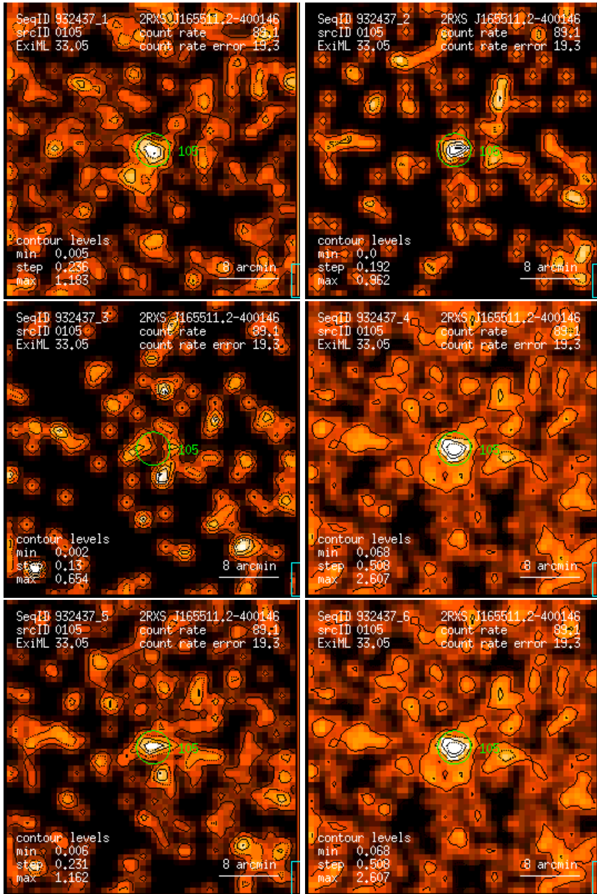
Figure 105: RASS 932437: detection 0105: band rate images, Gaussian filter: (1) PSPC channels 11 – 41, (2) 52 – 90, (3) 91 – 201, (4) 11 – 235, (5) 52 – 201, (6) 11 – 201. Broad band rates in counts/ks. Band rate contour levels in counts/ks/arcmin 2 .
