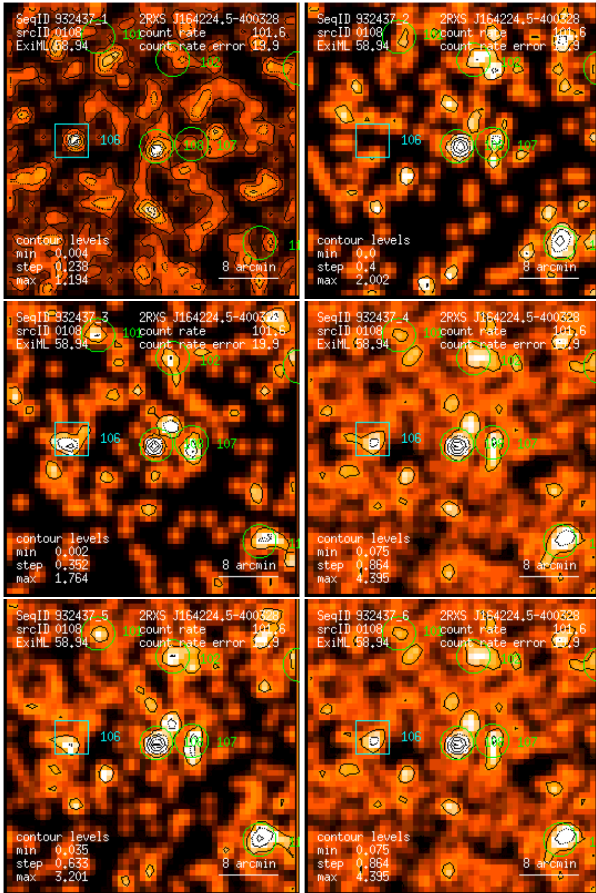
Figure 108: RASS 932437: detection 0108: band rate images, Gaussian filter: (1) PSPC channels 11 – 41, (2) 52 – 90, (3) 91 – 201, (4) 11 – 235, (5) 52 – 201, (6) 11 – 201. Broad band rates in counts/ks. Band rate contour levels in counts/ks/arcmin 2 .
