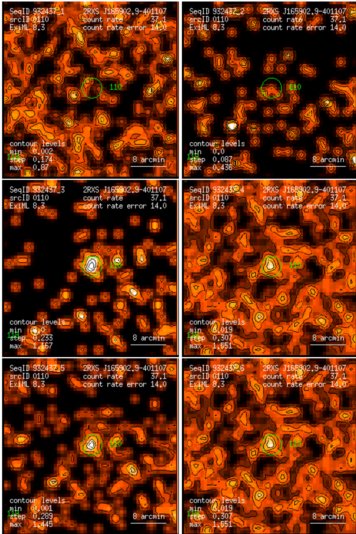
Figure 110: RASS 932437: detection 0110: band rate images, Gaussian filter: (1) PSPC channels 11 – 41, (2) 52 – 90, (3) 91 – 201, (4) 11 – 235, (5) 52 – 201, (6) 11 – 201. Broad band rates in counts/ks. Band rate contour levels in counts/ks/arcmin 2 .
