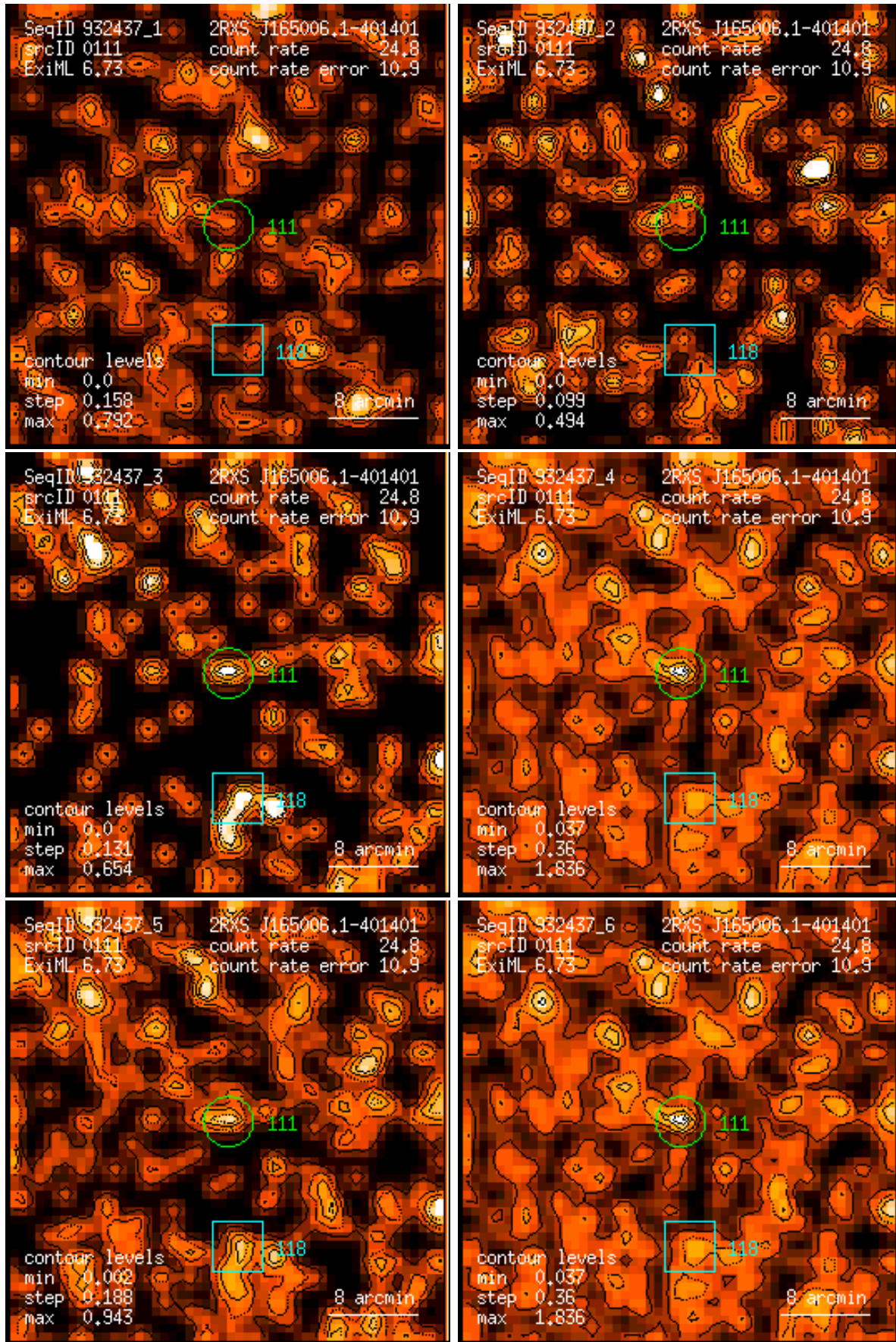
Figure 111: RASS 932437: detection 0111: band rate images, Gaussian filter: (1) PSPC channels 11 – 41, (2) 52 – 90, (3) 91 – 201, (4) 11 – 235, (5) 52 – 201, (6) 11 – 201. Broad band rates in counts/ks. Band rate contour levels in counts/ks/arcmin 2 .
