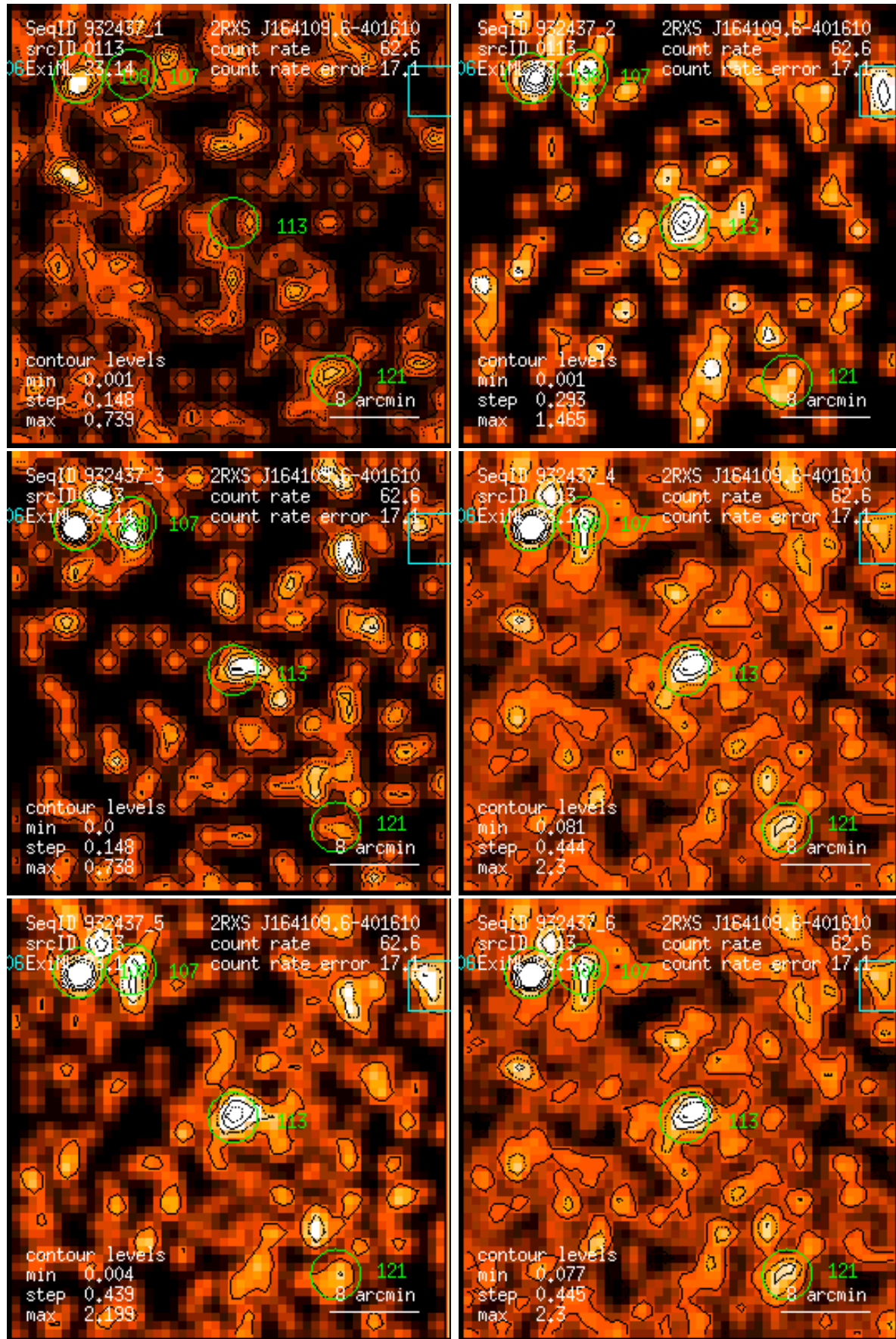
Figure 113: RASS 932437: detection 0113: band rate images, Gaussian filter: (1) PSPC channels 11 – 41, (2) 52 – 90, (3) 91 – 201, (4) 11 – 235, (5) 52 – 201, (6) 11 – 201. Broad band rates in counts/ks. Band rate contour levels in counts/ks/arcmin 2 .
