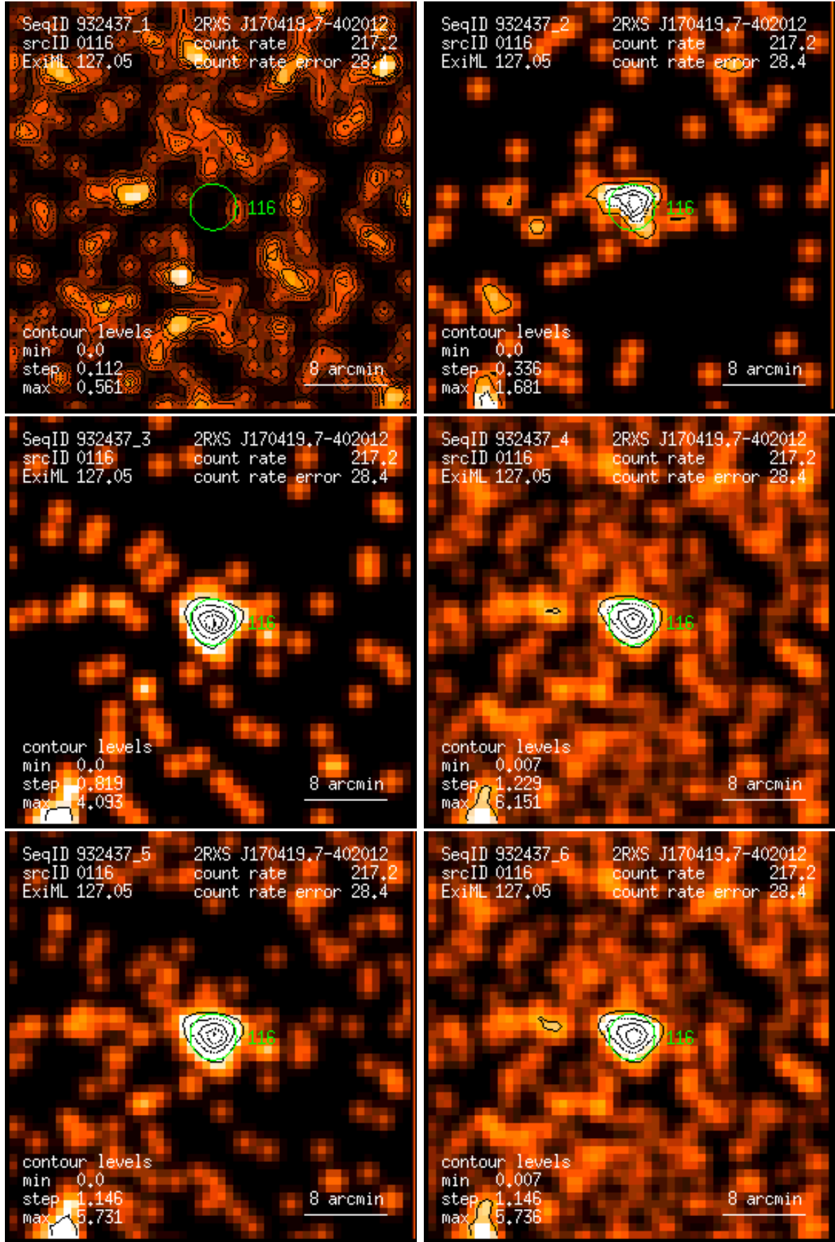
Figure 116: RASS 932437: detection 0116: band rate images, Gaussian filter: (1) PSPC channels 11 – 41, (2) 52 – 90, (3) 91 – 201, (4) 11 – 235, (5) 52 – 201, (6) 11 – 201. Broad band rates in counts/ks. Band rate contour levels in counts/ks/arcmin 2 .
