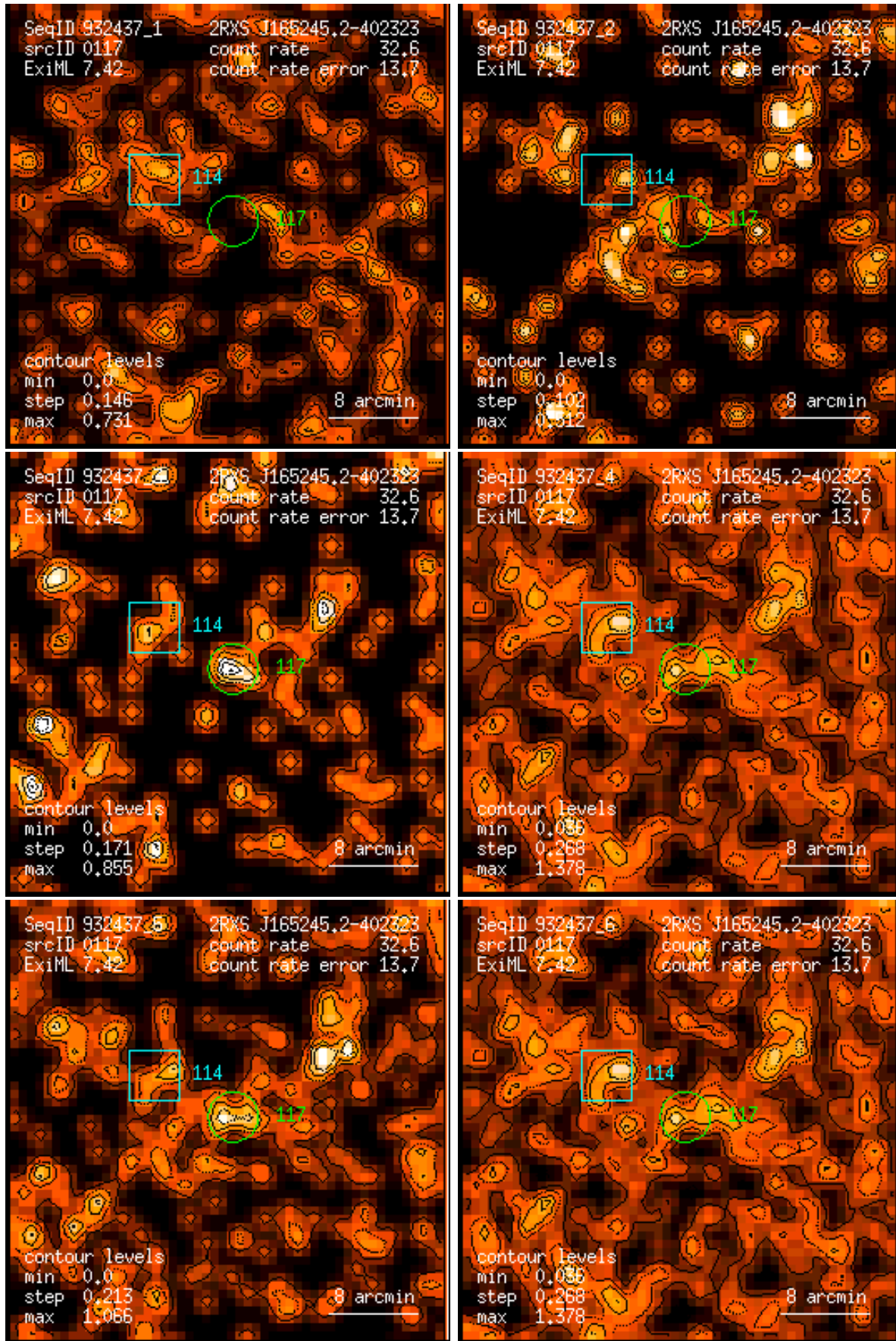
Figure 117: RASS 932437: detection 0117: band rate images, Gaussian filter: (1) PSPC channels 11 – 41, (2) 52 – 90, (3) 91 – 201, (4) 11 – 235, (5) 52 – 201, (6) 11 – 201. Broad band rates in counts/ks. Band rate contour levels in counts/ks/arcmin 2 .
