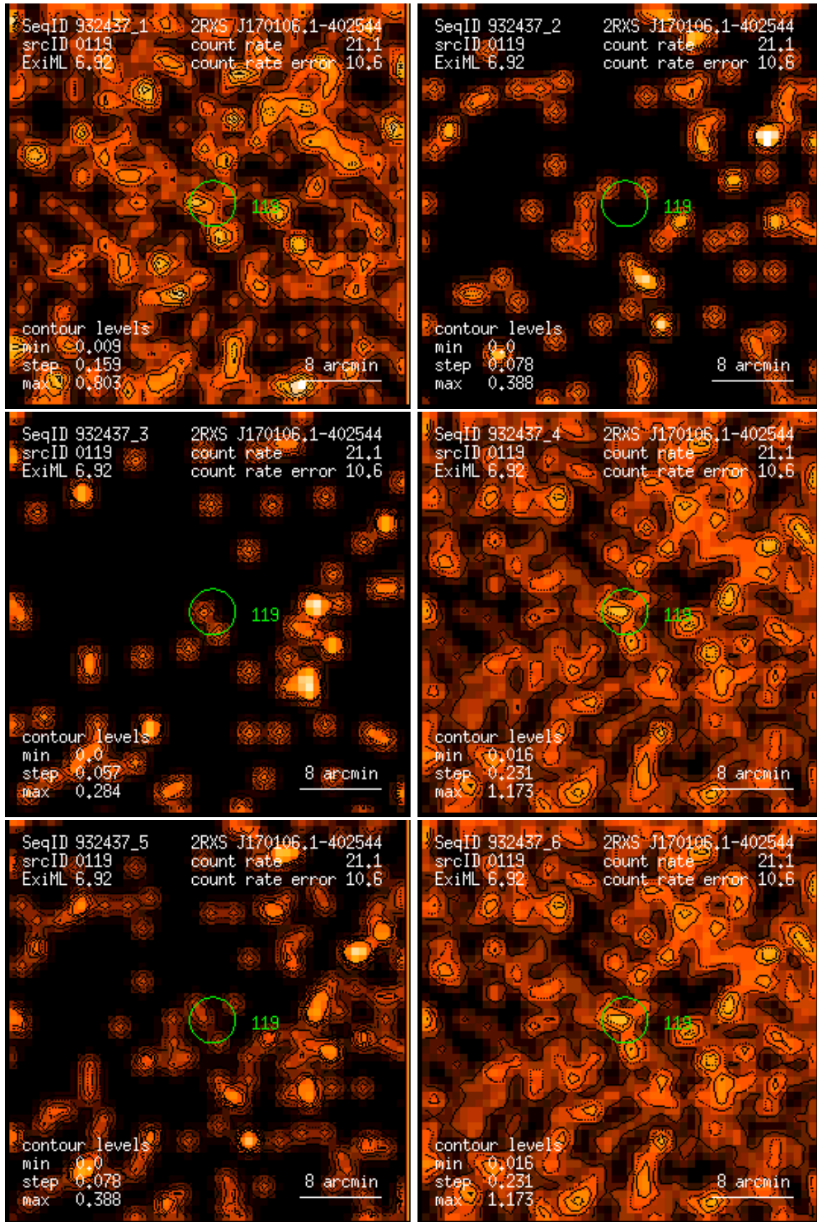
Figure 119: RASS 932437: detection 0119: band rate images, Gaussian filter: (1) PSPC channels 11 – 41, (2) 52 – 90, (3) 91 – 201, (4) 11 – 235, (5) 52 – 201, (6) 11 – 201. Broad band rates in counts/ks. Band rate contour levels in counts/ks/arcmin 2 .
