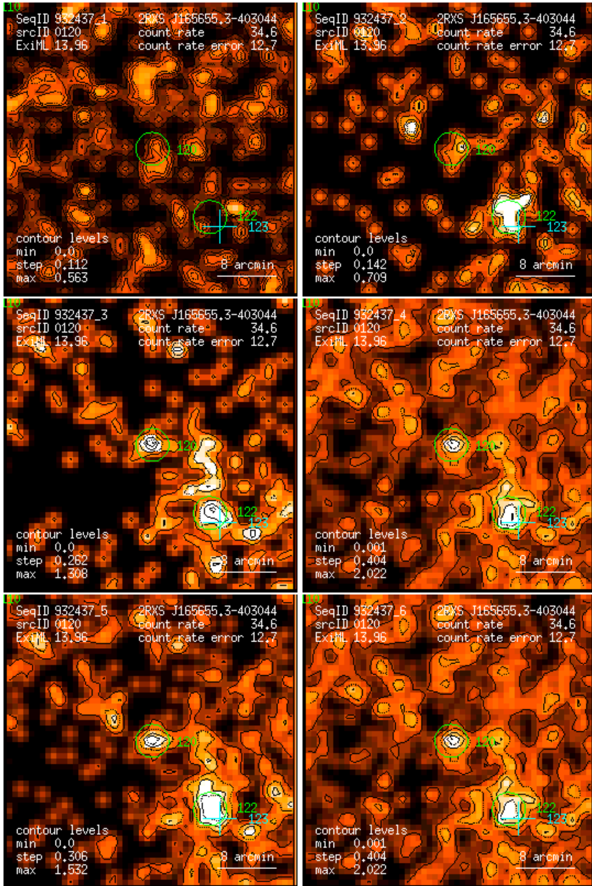
Figure 120: RASS 932437: detection 0120: band rate images, Gaussian filter: (1) PSPC channels 11 – 41, (2) 52 – 90, (3) 91 – 201, (4) 11 – 235, (5) 52 – 201, (6) 11 – 201. Broad band rates in counts/ks. Band rate contour levels in counts/ks/arcmin 2 .
