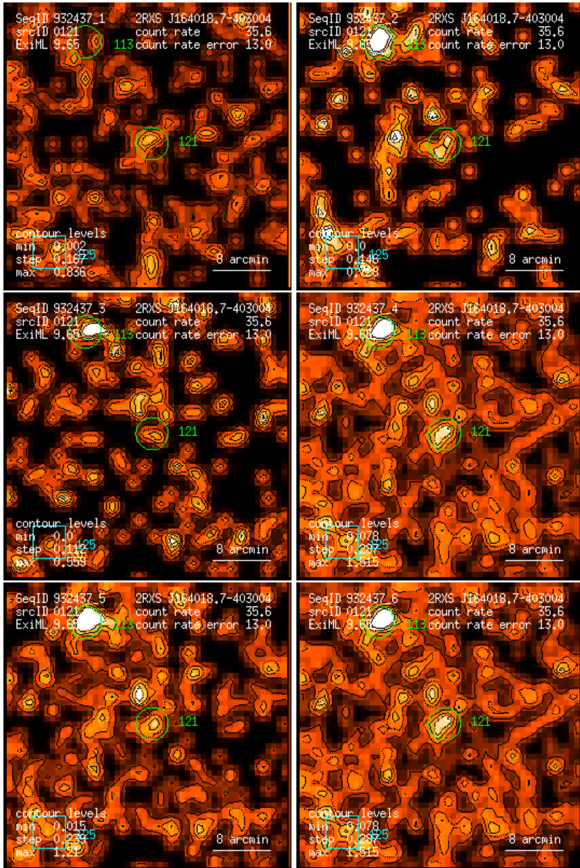
Figure 121: RASS 932437: detection 0121: band rate images, Gaussian filter: (1) PSPC channels 11 – 41, (2) 52 – 90, (3) 91 – 201, (4) 11 – 235, (5) 52 – 201, (6) 11 – 201. Broad band rates in counts/ks. Band rate contour levels in counts/ks/arcmin 2 .
