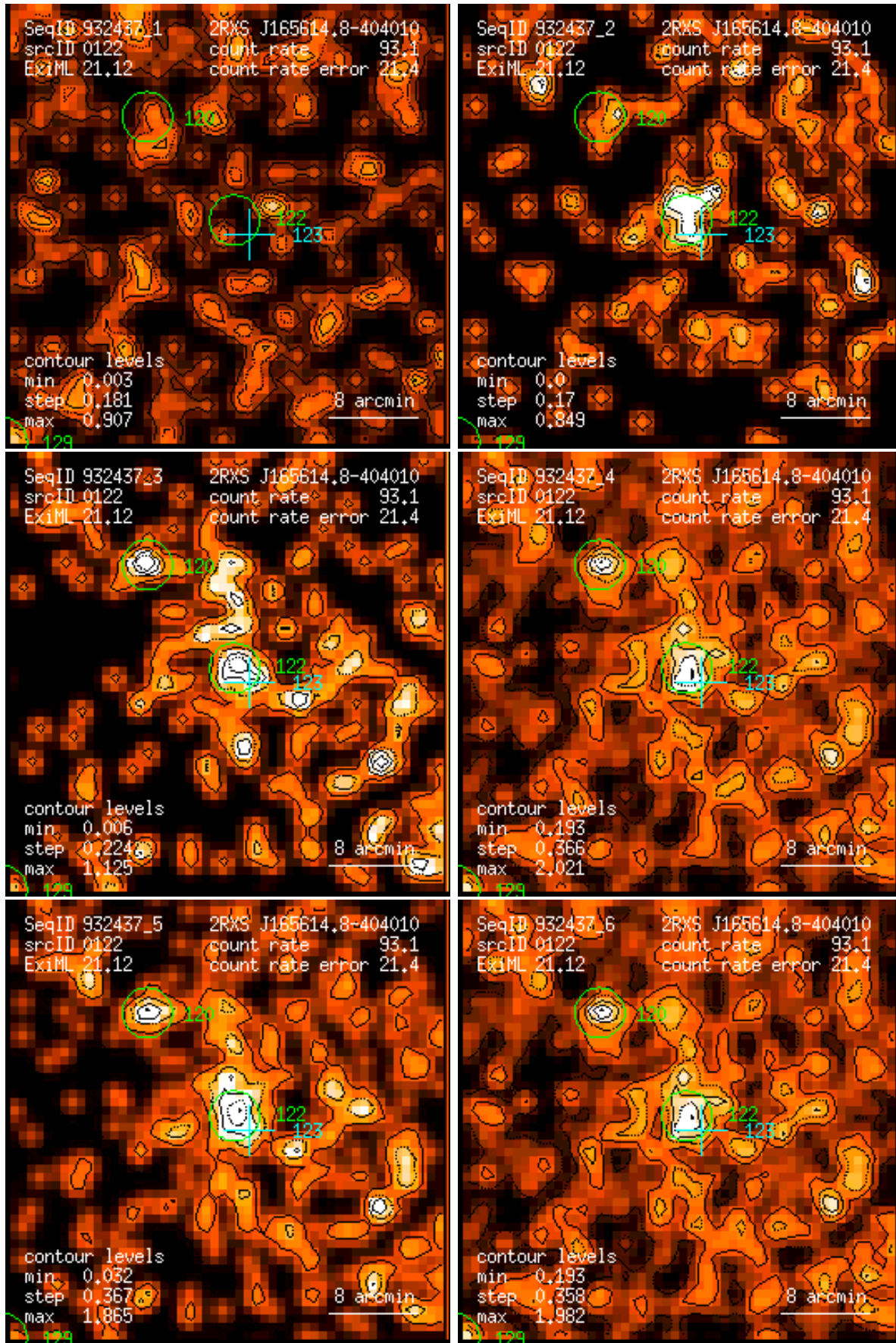
Figure 122: RASS 932437: detection 0122: band rate images, Gaussian filter: (1) PSPC channels 11 – 41, (2) 52 – 90, (3) 91 – 201, (4) 11 – 235, (5) 52 – 201, (6) 11 – 201. Broad band rates in counts/ks. Band rate contour levels in counts/ks/arcmin 2 .
