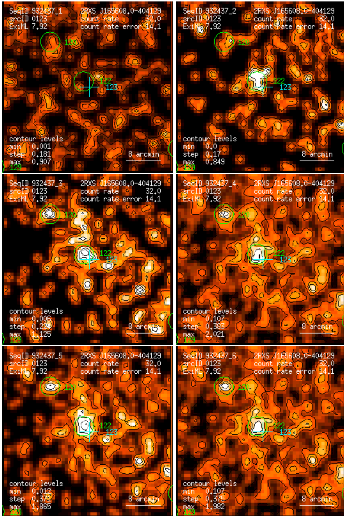
Figure 123: RASS 932437: detection 0123: band rate images, Gaussian filter: (1) PSPC channels 11 – 41, (2) 52 – 90, (3) 91 – 201, (4) 11 – 235, (5) 52 – 201, (6) 11 – 201. Broad band rates in counts/ks. Band rate contour levels in counts/ks/arcmin 2 .
