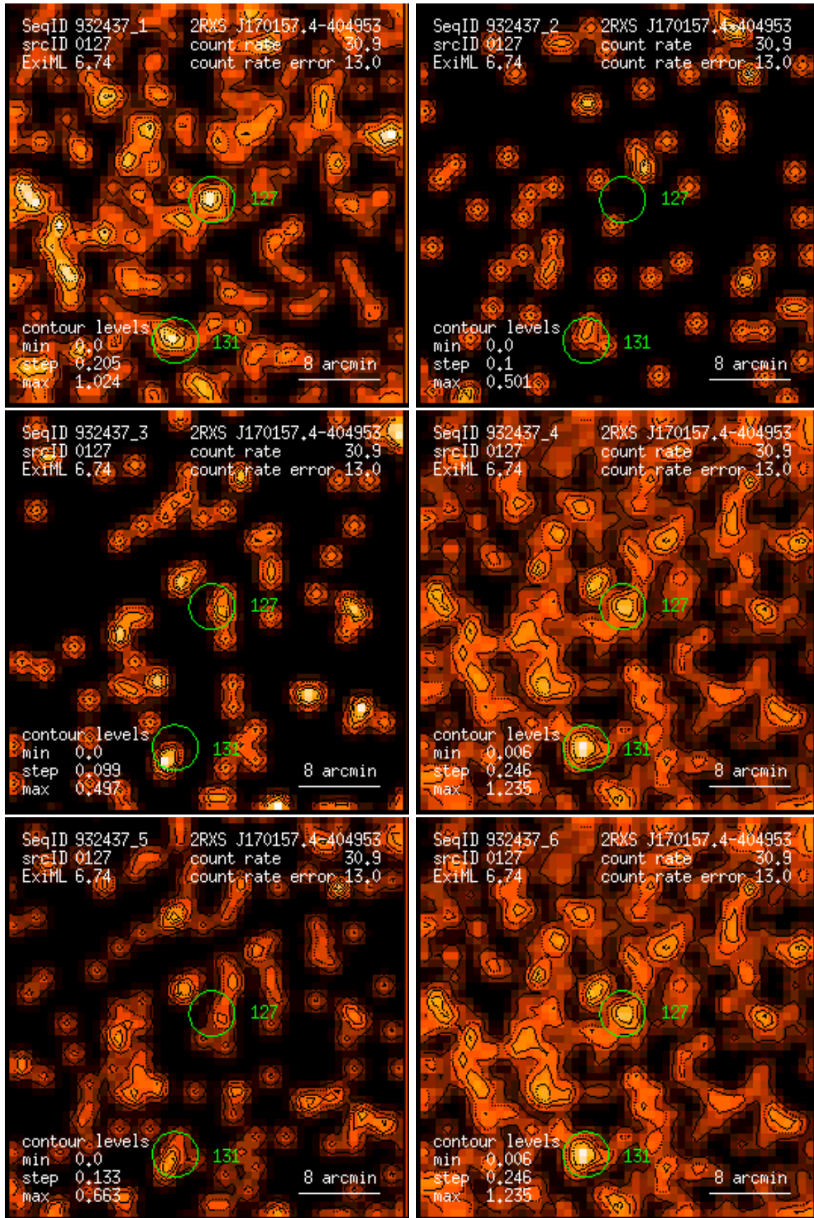
Figure 127: RASS 932437: detection 0127: band rate images, Gaussian filter: (1) PSPC channels 11 – 41, (2) 52 – 90, (3) 91 – 201, (4) 11 – 235, (5) 52 – 201, (6) 11 – 201. Broad band rates in counts/ks. Band rate contour levels in counts/ks/arcmin 2 .
