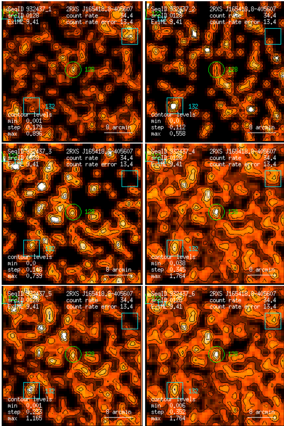
Figure 128: RASS 932437: detection 0128: band rate images, Gaussian filter: (1) PSPC channels 11 – 41, (2) 52 – 90, (3) 91 – 201, (4) 11 – 235, (5) 52 – 201, (6) 11 – 201. Broad band rates in counts/ks. Band rate contour levels in counts/ks/arcmin 2 .
