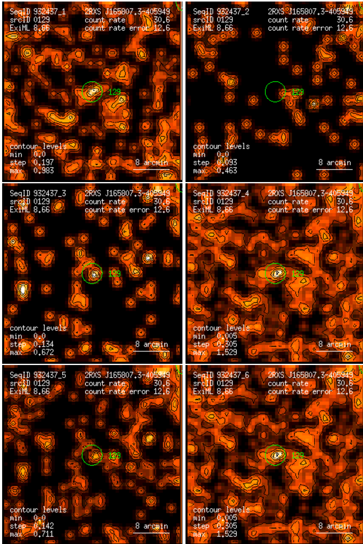
Figure 129: RASS 932437: detection 0129: band rate images, Gaussian filter: (1) PSPC channels 11 – 41, (2) 52 – 90, (3) 91 – 201, (4) 11 – 235, (5) 52 – 201, (6) 11 – 201. Broad band rates in counts/ks. Band rate contour levels in counts/ks/arcmin 2 .
