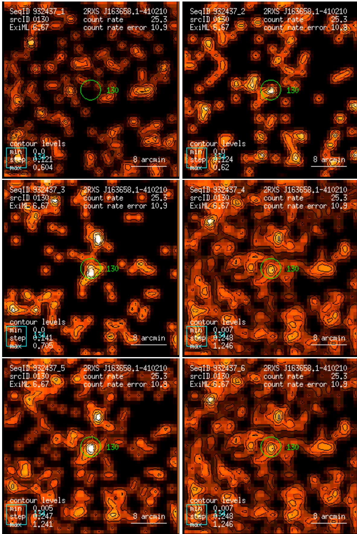
Figure 130: RASS 932437: detection 0130: band rate images, Gaussian filter: (1) PSPC channels 11 – 41, (2) 52 – 90, (3) 91 – 201, (4) 11 – 235, (5) 52 – 201, (6) 11 – 201. Broad band rates in counts/ks. Band rate contour levels in counts/ks/arcmin 2 .
