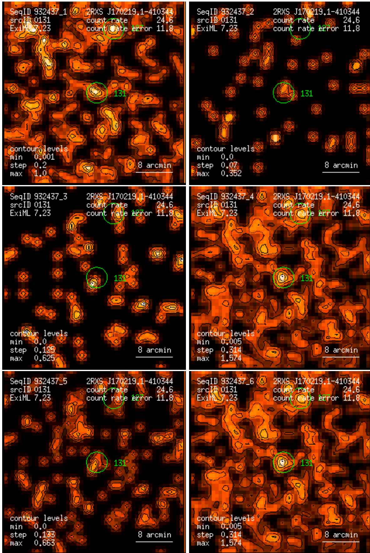
Figure 131: RASS 932437: detection 0131: band rate images, Gaussian filter: (1) PSPC channels 11 – 41, (2) 52 – 90, (3) 91 – 201, (4) 11 – 235, (5) 52 – 201, (6) 11 – 201. Broad band rates in counts/ks. Band rate contour levels in counts/ks/arcmin 2 .
