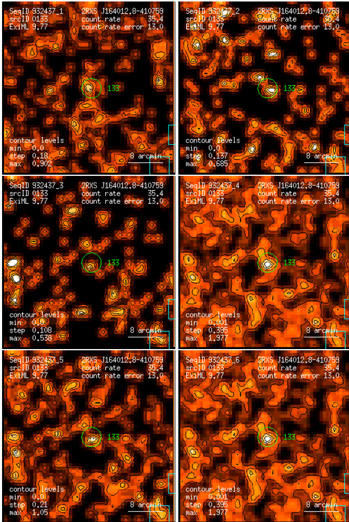
Figure 133: RASS 932437: detection 0133: band rate images, Gaussian filter: (1) PSPC channels 11 – 41, (2) 52 – 90, (3) 91 – 201, (4) 11 – 235, (5) 52 – 201, (6) 11 – 201. Broad band rates in counts/ks. Band rate contour levels in counts/ks/arcmin 2 .
