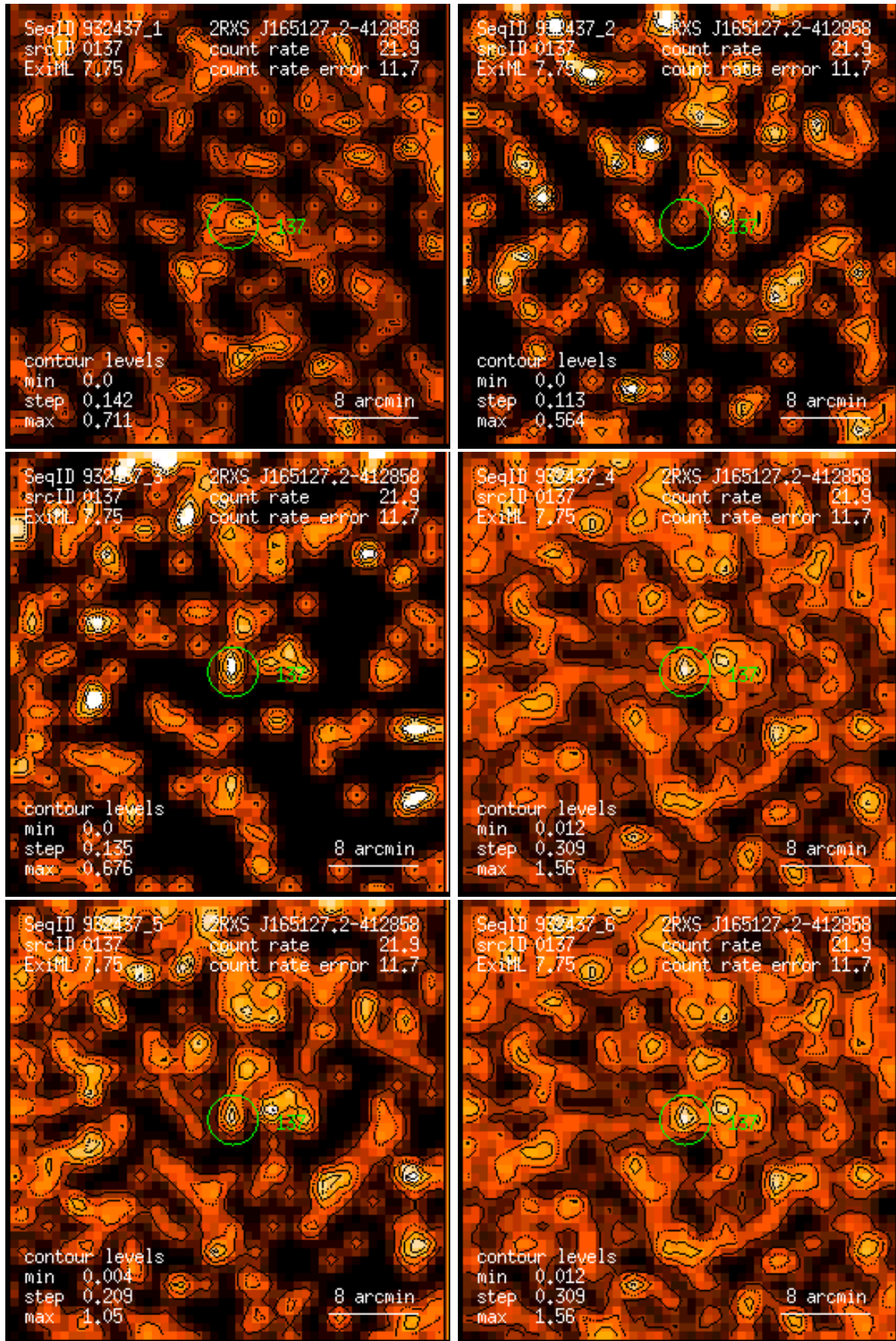
Figure 137: RASS 932437: detection 0137: band rate images, Gaussian filter: (1) PSPC channels 11 – 41, (2) 52 – 90, (3) 91 – 201, (4) 11 – 235, (5) 52 – 201, (6) 11 – 201. Broad band rates in counts/ks. Band rate contour levels in counts/ks/arcmin 2 .
