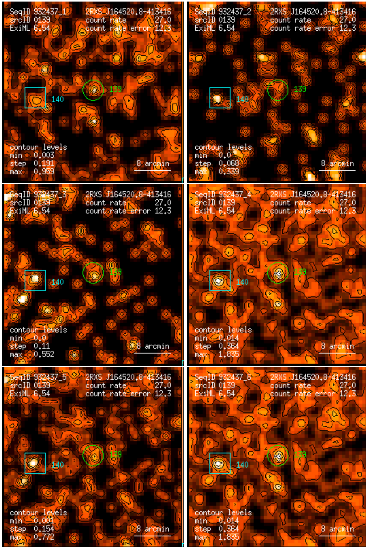
Figure 139: RASS 932437: detection 0139: band rate images, Gaussian filter: (1) PSPC channels 11 – 41, (2) 52 – 90, (3) 91 – 201, (4) 11 – 235, (5) 52 – 201, (6) 11 – 201. Broad band rates in counts/ks. Band rate contour levels in counts/ks/arcmin 2 .
