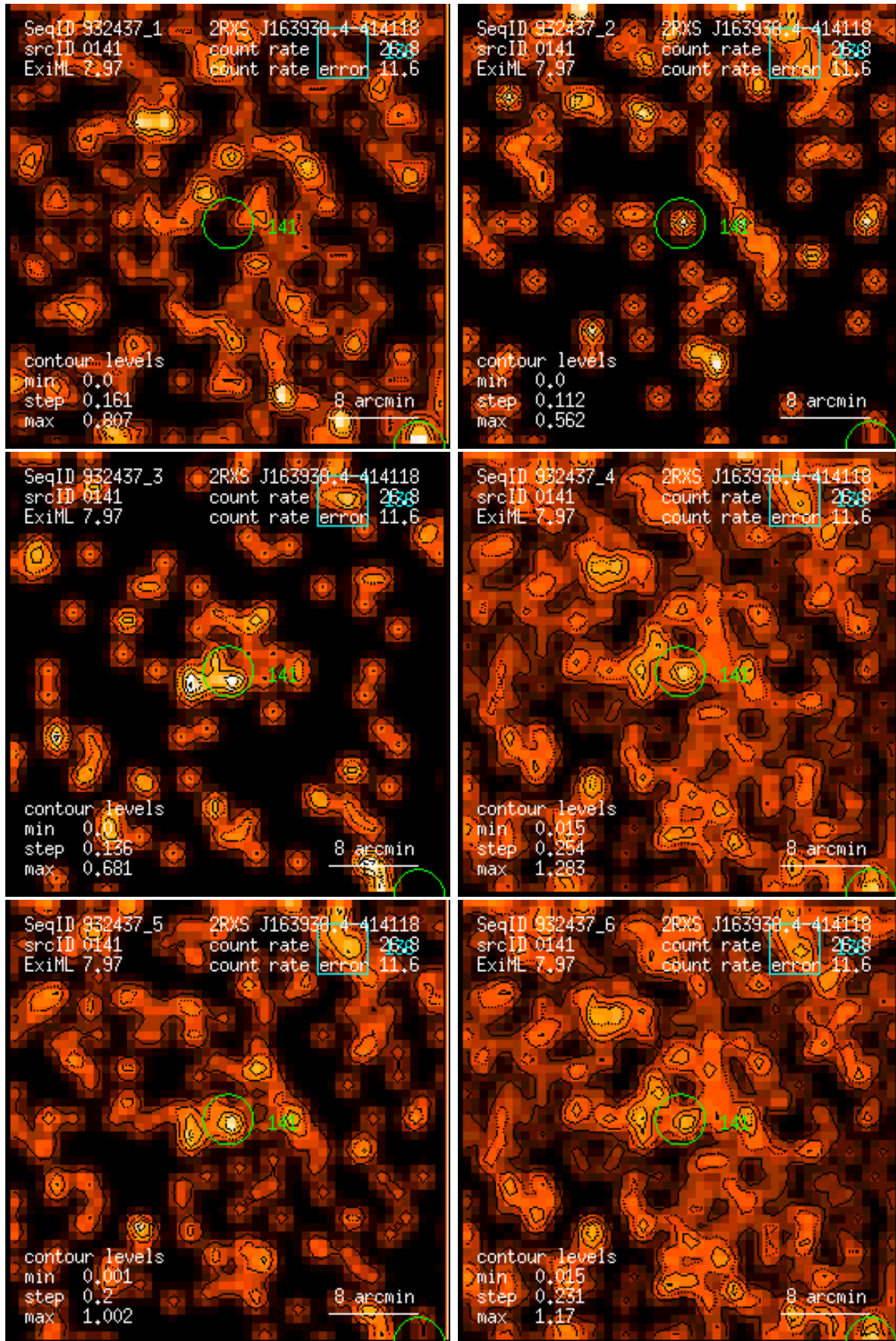
Figure 141: RASS 932437: detection 0141: band rate images, Gaussian filter: (1) PSPC channels 11 – 41, (2) 52 – 90, (3) 91 – 201, (4) 11 – 235, (5) 52 – 201, (6) 11 – 201. Broad band rates in counts/ks. Band rate contour levels in counts/ks/arcmin 2 .
